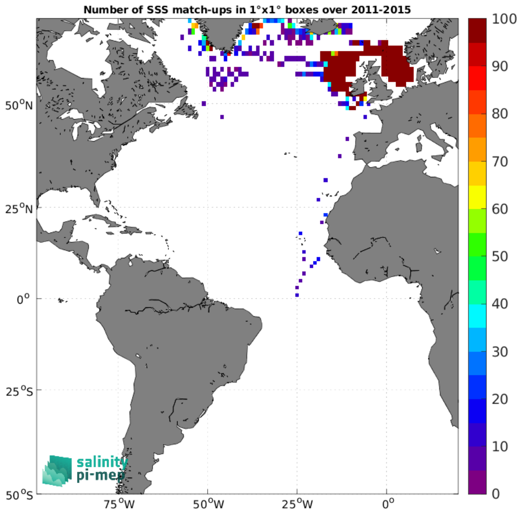
Figure 4: Number of SSS match-ups between ICES SSS and the Aquarius SSS L3 OR v5 - Monthly - Rain mask (NASA-GSFC) SSS product for the Atlantic Ocean Pi-MEP region over 1°×1° boxes and for the full satellite product period.
