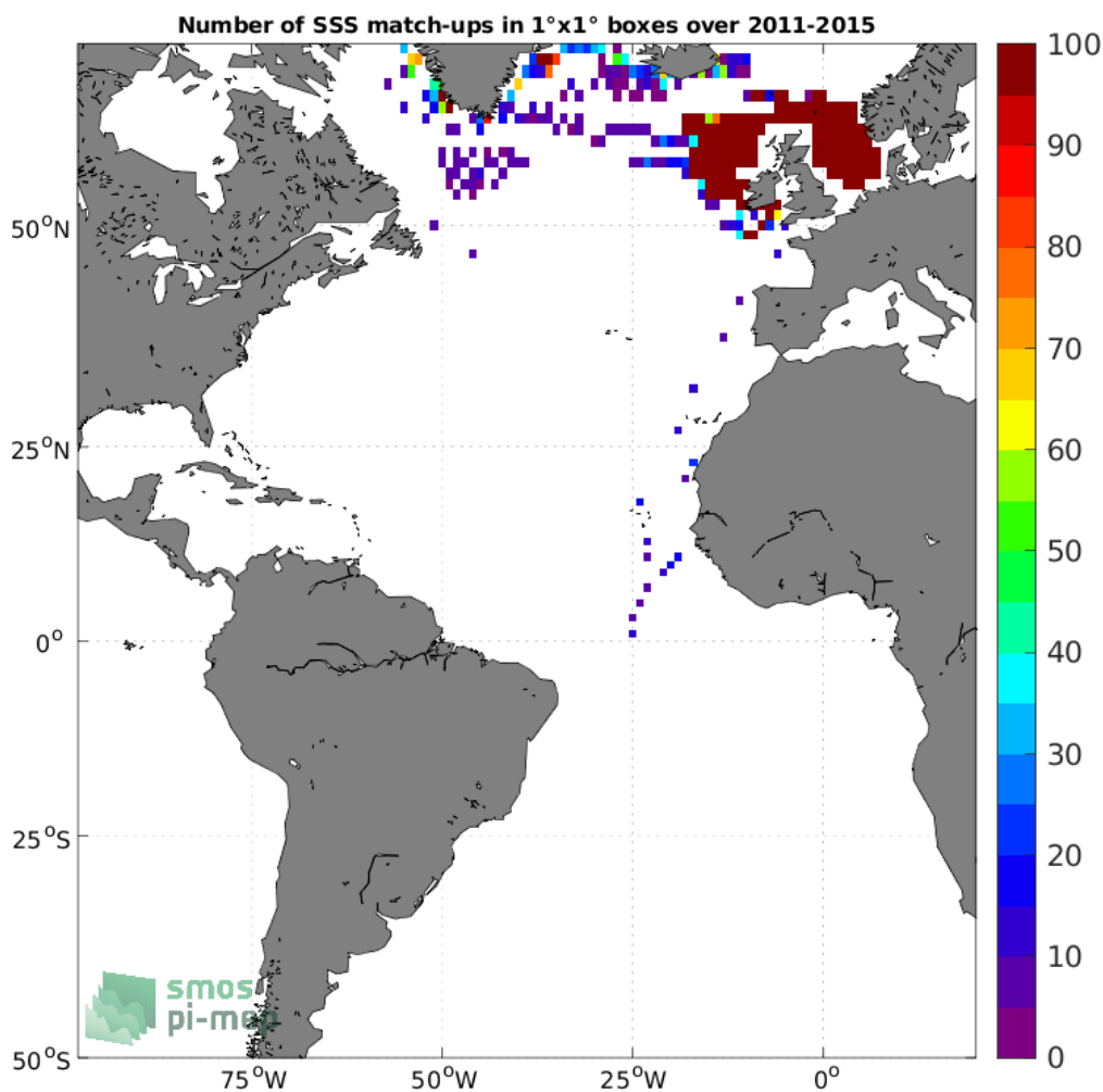
Figure 4: Number of SSS match-ups between ICES SSS and the Aquarius SSS L3 OR v5 - Monthly - Rain mask (NASA-GSFC) SSS product for the Atlantic Ocean Pi-MEP region over 1°x1° boxes and for the full satellite product period.
