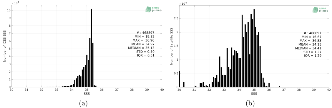
Figure 2: Histograms of SSS from ICES (a) and Aquarius SSS L3 OR v5 - Monthly - Rain mask (NASA-GSFC) (b) considering all match-up pairs per bins of 0.1 over the Atlantic Ocean Pi-MEP region and for the full satellite product period.
