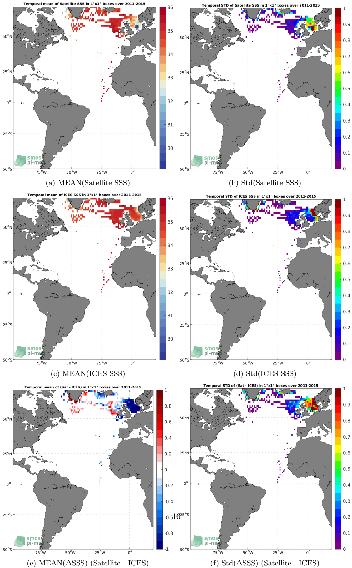
Figure 6: Temporal mean (left) and Std (right) of SSS from Aquarius SSS L3 OR v5 - Monthly - Rain mask (NASA-GSFC) (top), ICES (middle), and of \Delta SSS (Satellite - ICES). Only match-up pairs are used to generate these maps.
