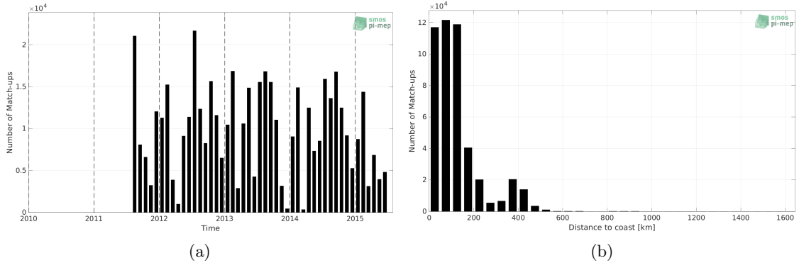
Figure 1: Number of match-ups between ICES and Aquarius SSS L3 OR v5 - Monthly - Rain mask (NASA-GSFC) SSS as a function of time (a) and as function of the distance to coast (b) over the Atlantic Ocean Pi-MEP region and for the full satellite product period.
