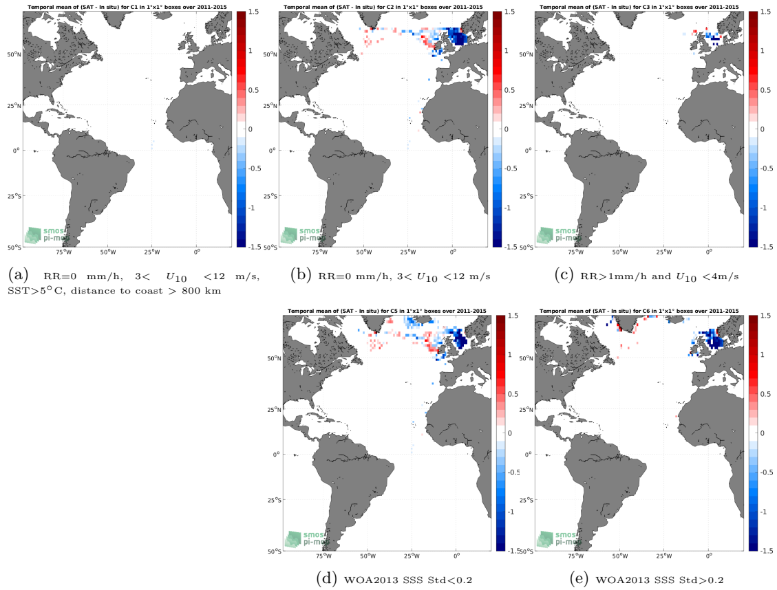
Figure 12: Temporal mean gridded over spatial boxes of size 1^\circ \times 1^\circ of \Delta SSS (Aquarius SSS L3 OR v5 - Monthly - Rain mask (NASA-GSFC) - ICES) for 5 different subdatasets corresponding to:RR=0 mm/h, 3 < U_{10} < 12 m/s, SST >5^\circ\text{C} , distance to coast > 800 km (a), RR=0 mm/h, 3 < U_{10} < 12 m/s (b), RR >1 mm/h and U_{10} < 4 m/s (c), WOA2013 SSS Std <0.2 (d), WOA2013 SSS Std >0.2 (e).
