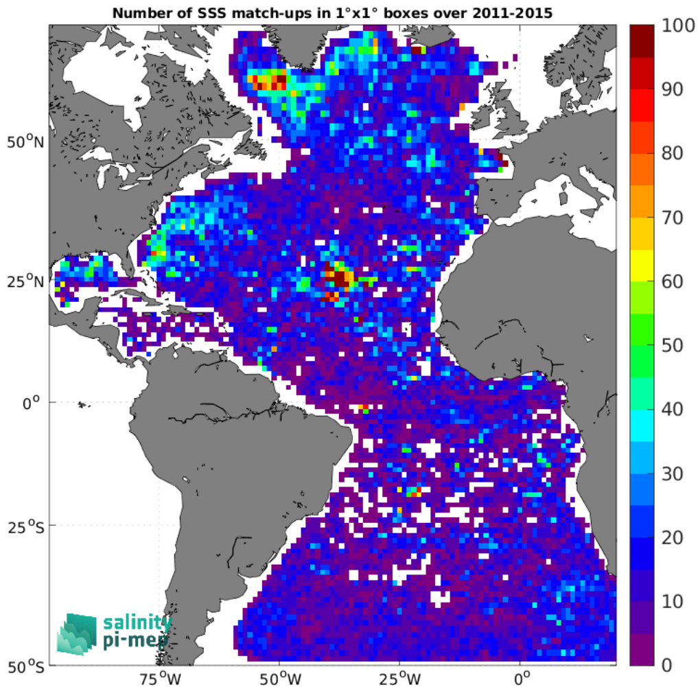
Figure 4: Number of SSS match-ups between Argo SSS and the Aquarius SSS L3 OR v5 - Monthly - Rain mask (NASA-GSFC) SSS product for the Atlantic Ocean Pi-MEP region over 1°×1° boxes and for the full satellite product period.
