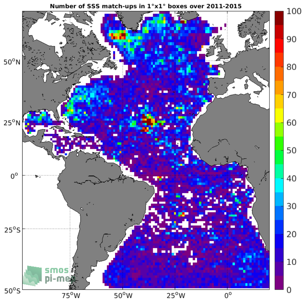
Figure 4: Number of SSS match-ups between Argo SSS and the Aquarius SSS L3 OR v5 - Monthly - Rain mask (NASA-GSFC) SSS product for the Atlantic Ocean Pi-MEP region over 1°x1° boxes and for the full satellite product period.
