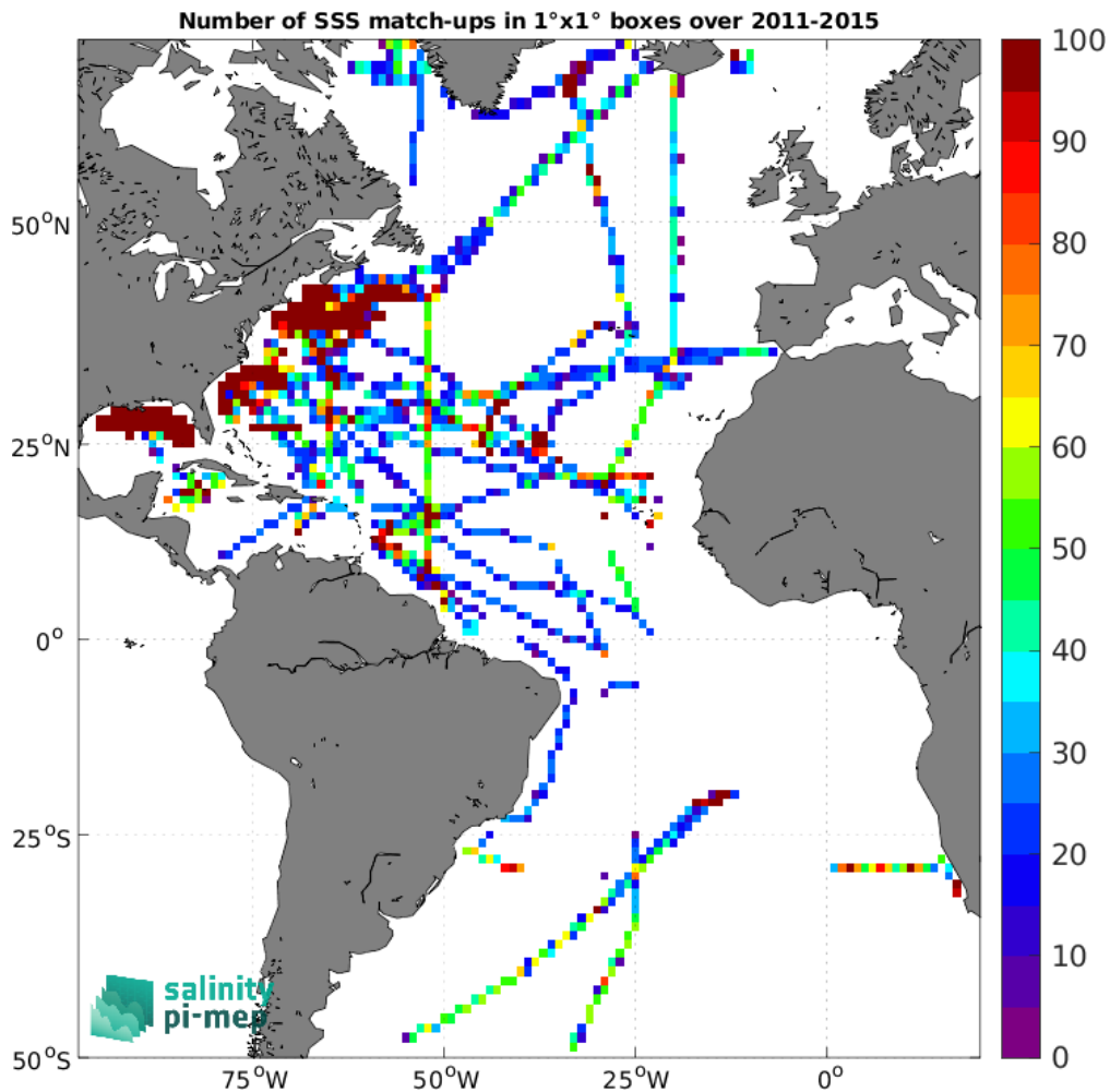
Figure 5: Number of SSS match-ups between TSG (SAMOS) SSS and the Aquarius SSS L3 CAP v5 - 7-Day running (JPL) SSS product for the Atlantic Ocean Pi-MEP region over 1^\circ \times 1^\circ boxes and for the full satellite product period.
