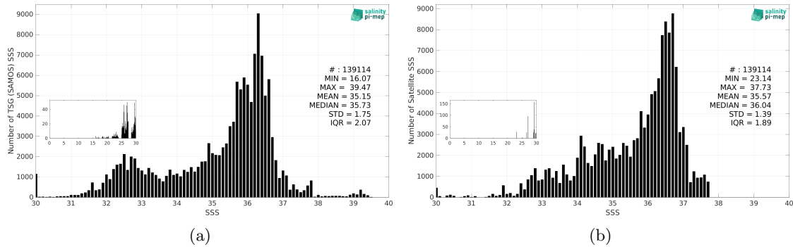
Figure 3: Histograms of SSS from TSG (SAMOS) (a) and Aquarius SSS L3 CAP v5 - 7-Day running (JPL) (b) considering all match-up pairs per bins of 0.1 over the Atlantic Ocean Pi-MEP region and for the full satellite product period.
