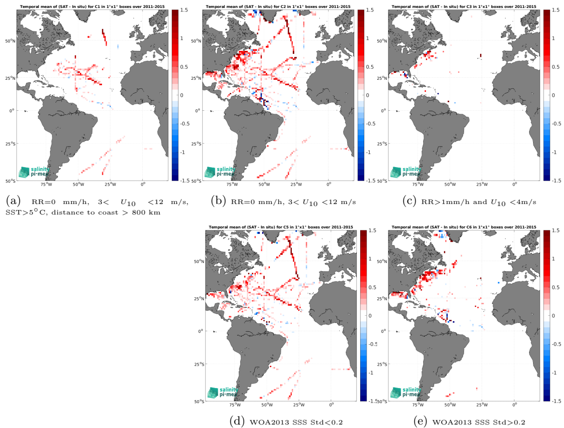
Figure 14: Temporal mean gridded over spatial boxes of size 1^\circ \times 1^\circ of \Delta\text{SSS} (Aquarius SSS L3 CAP v5 - 7-Day running (JPL) - TSG (SAMOS)) for 5 different subdatasets corresponding to:RR=0 mm/h, 3 < U_{10} < 12 m/s, SST>5°C, distance to coast > 800 km (a), RR=0 mm/h, 3 < U_{10} < 12 m/s (b), RR>1mm/h and U_{10} < 4 m/s (c), WOA2013 SSS Std<0.2 (d), WOA2013 SSS Std>0.2 (e).
