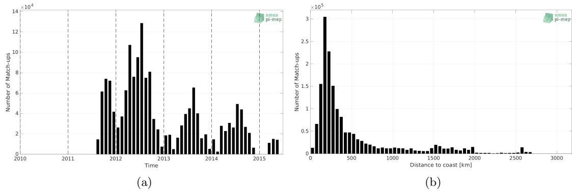
Figure 1: Number of match-ups between TSG (SAMOS) and Aquarius SSS L3 CAP v5 - 7-Day running (JPL) SSS as a function of time (a) and as function of the distance to coast (b) over the Atlantic Ocean Pi-MEP region and for the full satellite product period.
