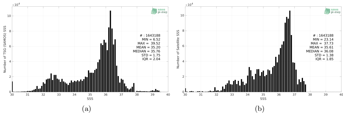
Figure 2: Histograms of SSS from TSG (SAMOS) (a) and Aquarius SSS L3 CAP v5 - 7-Day running (JPL) (b) considering all match-up pairs per bins of 0.1 over the Atlantic Ocean Pi-MEP region and for the full satellite product period.
