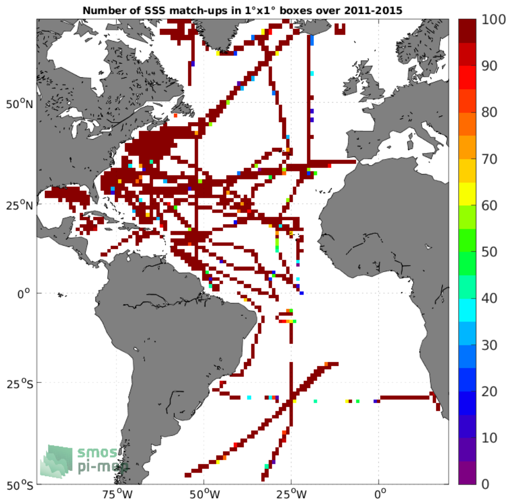
Figure 4: Number of SSS match-ups between TSG (SAMOS) SSS and the Aquarius SSS L3 CAP v5 - 7-Day running (JPL) SSS product for the Atlantic Ocean Pi-MEP region over 1^\circ \times 1^\circ boxes and for the full satellite product period.
