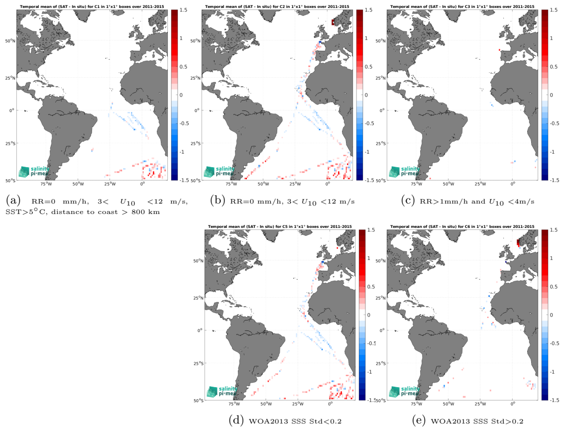
Figure 14: Temporal mean gridded over spatial boxes of size 1^\circ \times 1^\circ of \Delta SSS (Aquarius SSS L3 CAP v5 - 7-Day running (JPL) - TSG (Polarstern)) for 5 different subdatasets corresponding to:RR=0 mm/h, 3 < U_{10} < 12 m/s, SST>5°C, distance to coast > 800 km (a), RR=0 mm/h, 3 < U_{10} < 12 m/s (b), RR>1mm/h and U_{10} < 4 m/s (c), WOA2013 SSS Std<0.2 (d), WOA2013 SSS Std>0.2 (e).
