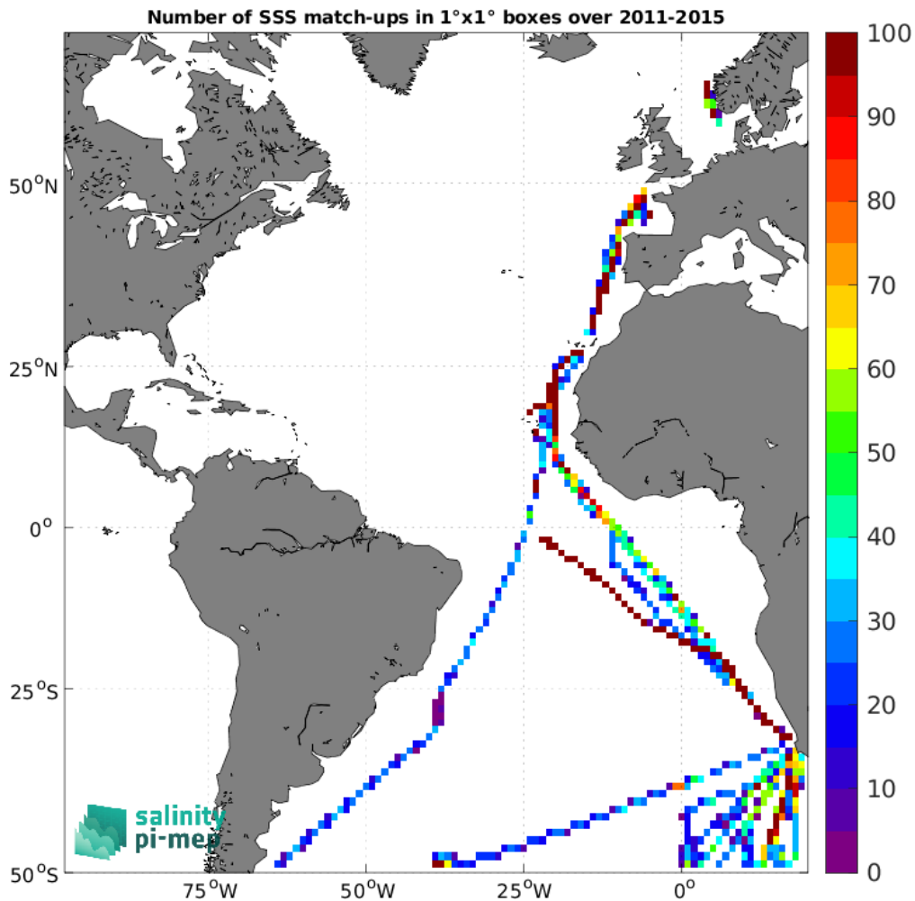
Figure 5: Number of SSS match-ups between TSG (Polarstern) SSS and the Aquarius SSS L3 CAP v5 - 7-Day running (JPL) SSS product for the Atlantic Ocean Pi-MEP region over 1°x1° boxes and for the full satellite product period.
