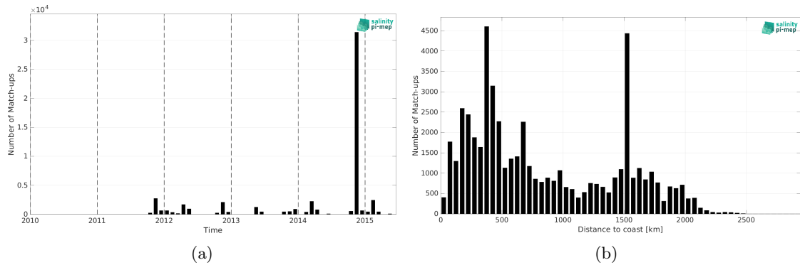
Figure 2: Number of match-ups between TSG (Polarstern) and Aquarius SSS L3 CAP v5 - 7-Day running (JPL) SSS as a function of time (a) and as function of the distance to coast (b) over the Atlantic Ocean Pi-MEP region and for the full satellite product period.
