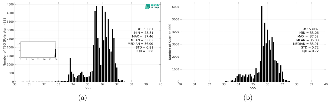
Figure 3: Histograms of SSS from TSG (Polarstern) (a) and Aquarius SSS L3 CAP v5 - 7-Day running (JPL) (b) considering all match-up pairs per bins of 0.1 over the Atlantic Ocean Pi-MEP region and for the full satellite product period.
