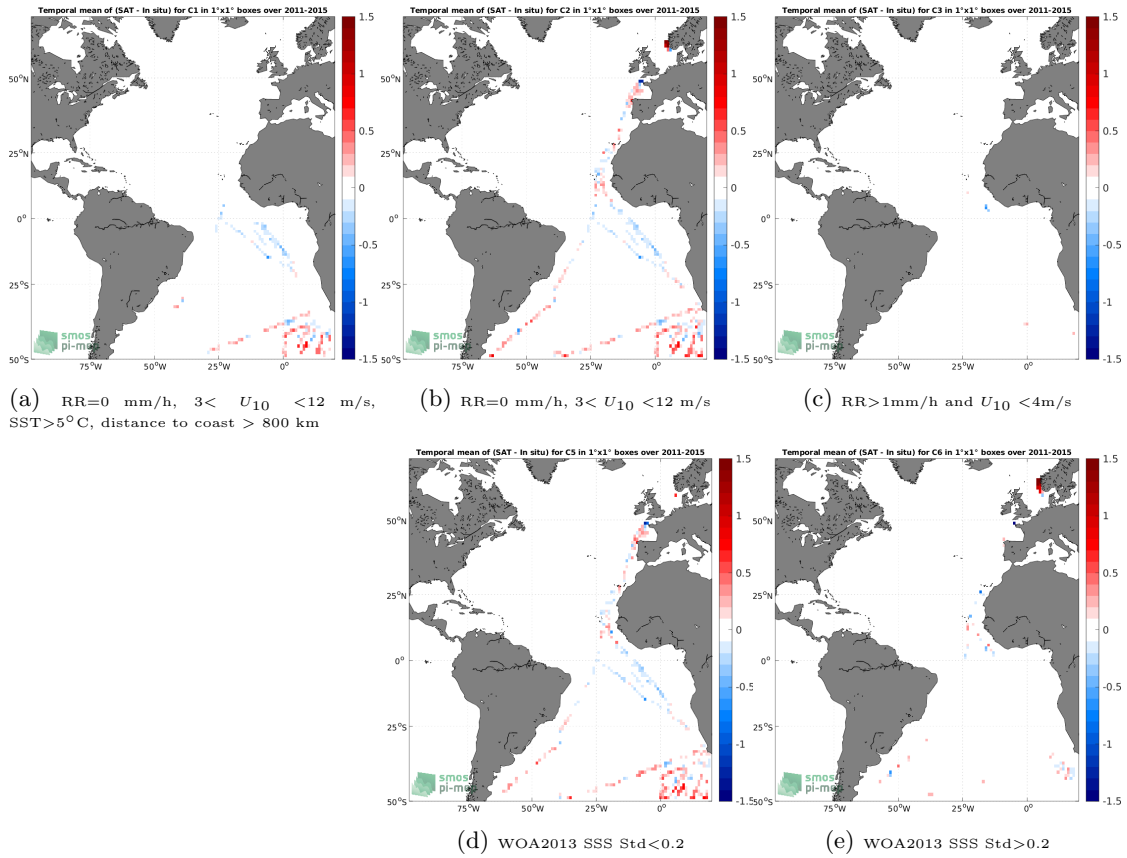
Figure 12: Temporal mean gridded over spatial boxes of size 1^\circ \times 1^\circ of \Delta SSS (Aquarius SSS L3 CAP v5 - 7-Day running (JPL) - TSG (Polarstern)) for 5 different subdatasets corresponding to:RR=0 mm/h, 3 < U_{10} < 12 m/s, SST >5^\circ\text{C} , distance to coast > 800 km (a), RR=0 mm/h, 3 < U_{10} < 12 m/s (b), RR >1 mm/h and U_{10} < 4 m/s (c), WOA2013 SSS Std <0.2 (d), WOA2013 SSS Std >0.2 (e).
