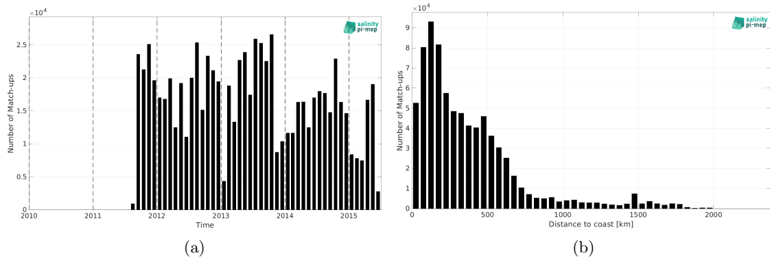
Figure 2: Number of match-ups between TSG (LEGOS-DM) and Aquarius SSS L3 CAP v5 - 7-Day running (JPL) SSS as a function of time (a) and as function of the distance to coast (b) over the Atlantic Ocean Pi-MEP region and for the full satellite product period.
