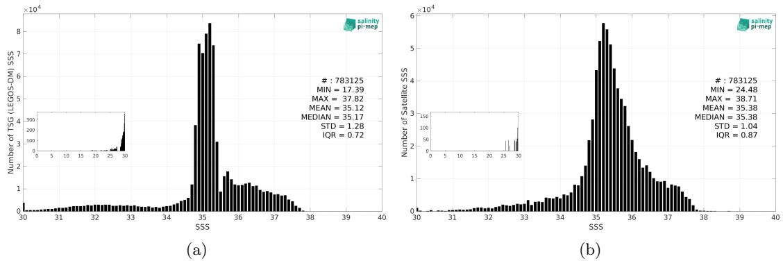
Figure 3: Histograms of SSS from TSG (LEGOS-DM) (a) and Aquarius SSS L3 CAP v5 - 7-Day running (JPL) (b) considering all match-up pairs per bins of 0.1 over the Atlantic Ocean Pi-MEP region and for the full satellite product period.
