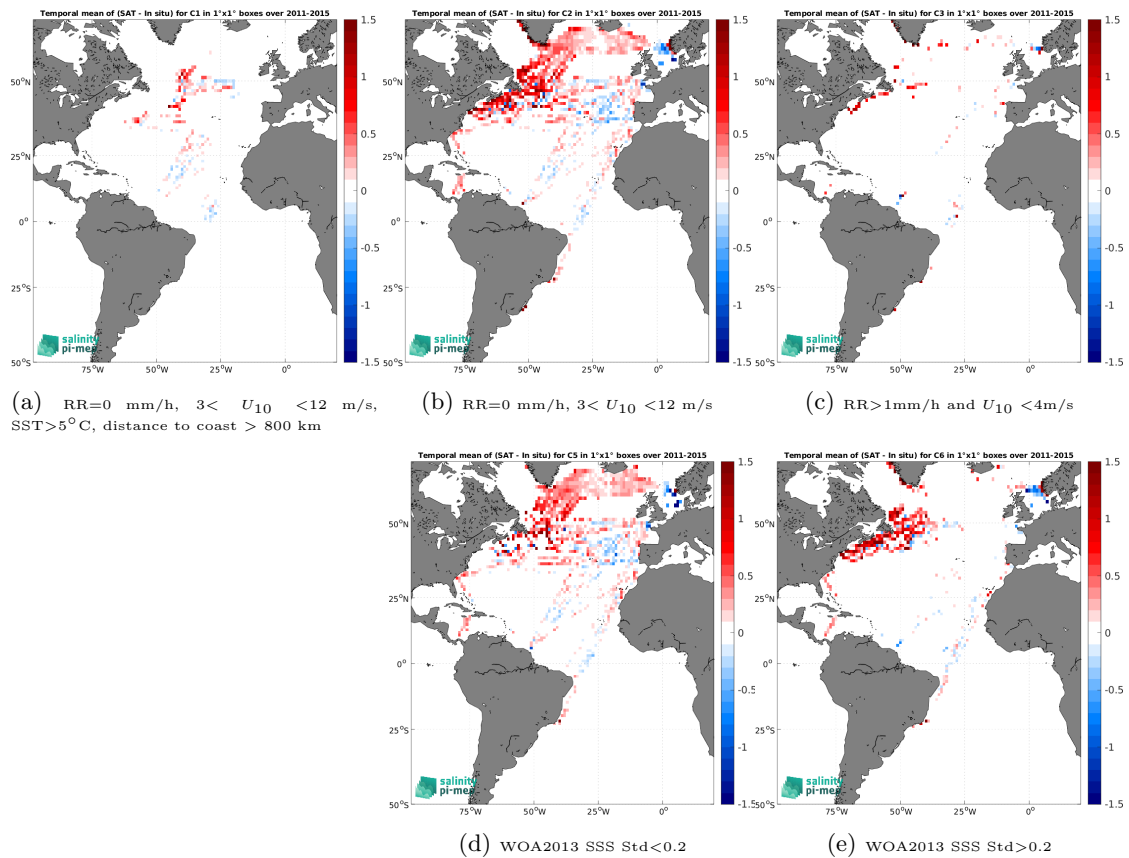
Figure 14: Temporal mean gridded over spatial boxes of size 1^\circ \times 1^\circ of \Delta\text{SSS} (Aquarius SSS L3 CAP v5 - 7-Day running (JPL) - TSG (LEGOS-DM)) for 5 different subdatasets corresponding to:RR=0 mm/h, 3 < U_{10} < 12 m/s, SST>5°C, distance to coast > 800 km (a), RR=0 mm/h, 3 < U_{10} < 12 m/s (b), RR>1mm/h and U_{10} < 4 m/s (c), WOA2013 SSS Std<0.2 (d), WOA2013 SSS Std>0.2 (e).
