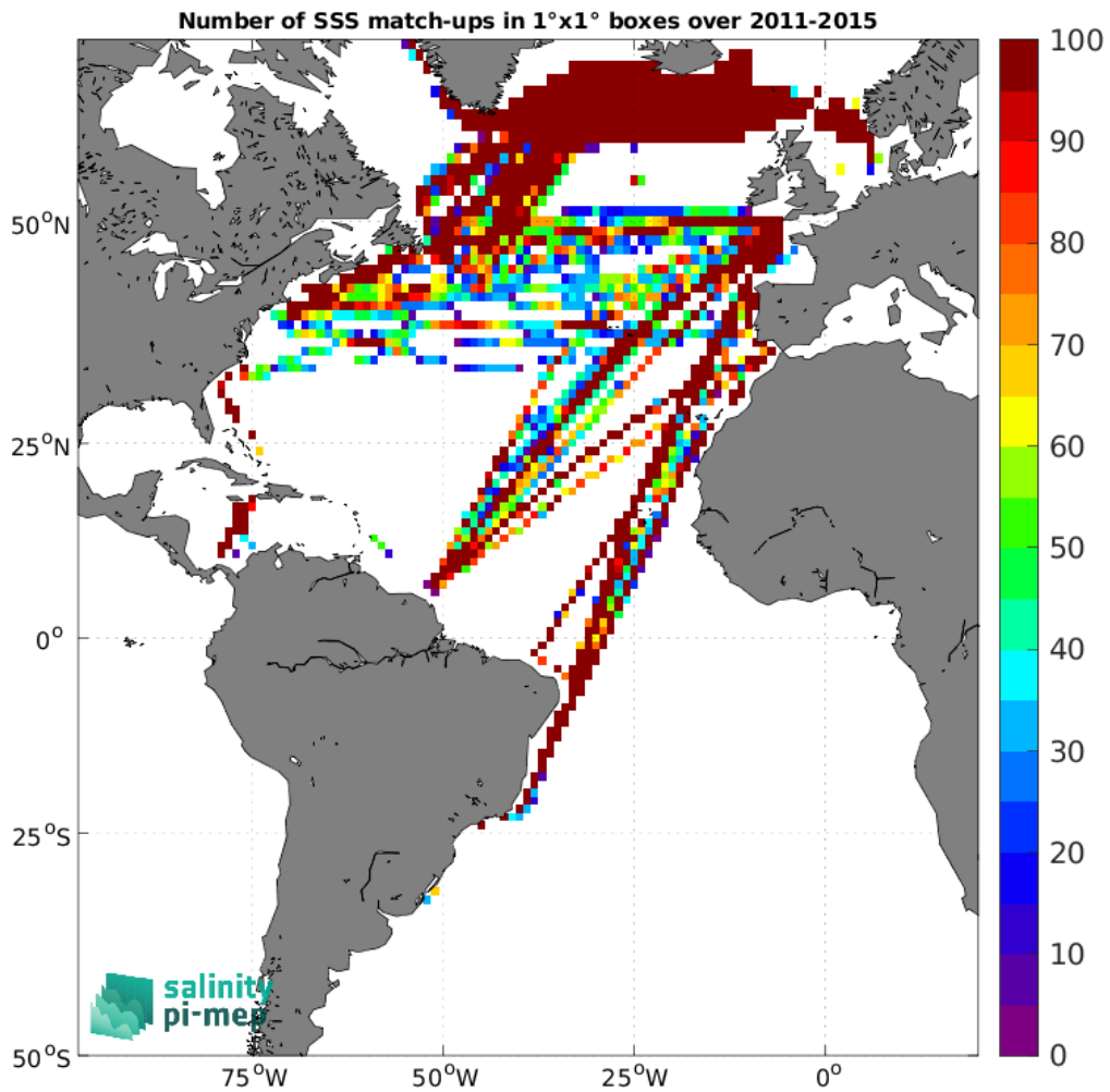
Figure 5: Number of SSS match-ups between TSG (LEGOS-DM) SSS and the Aquarius SSS L3 CAP v5 - 7-Day running (JPL) SSS product for the Atlantic Ocean Pi-MEP region over 1^\circ \times 1^\circ boxes and for the full satellite product period.
