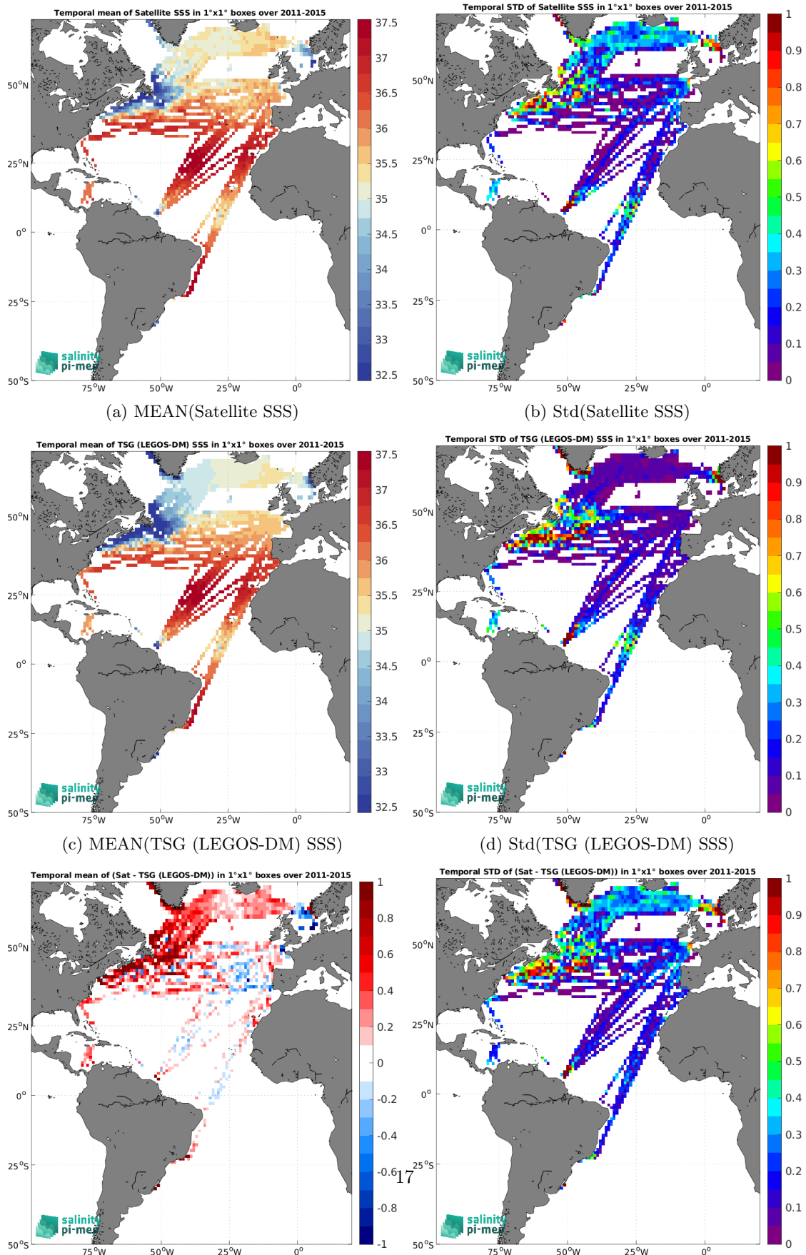
(e) MEAN( \Delta SSS) (Satellite - TSG (LEGOS-DM)) (f) Std( \Delta SSS) (Satellite - TSG (LEGOS-DM)) Figure 6: Temporal mean (left) and Std (right) of SSS from Aquarius SSS L3 CAP v5 - 7-Day running (JPL) (top), TSG (LEGOS-DM) (middle), and of \Delta SSS (Satellite - TSG (LEGOS-DM)). Only match-up pairs are used to generate these maps.
