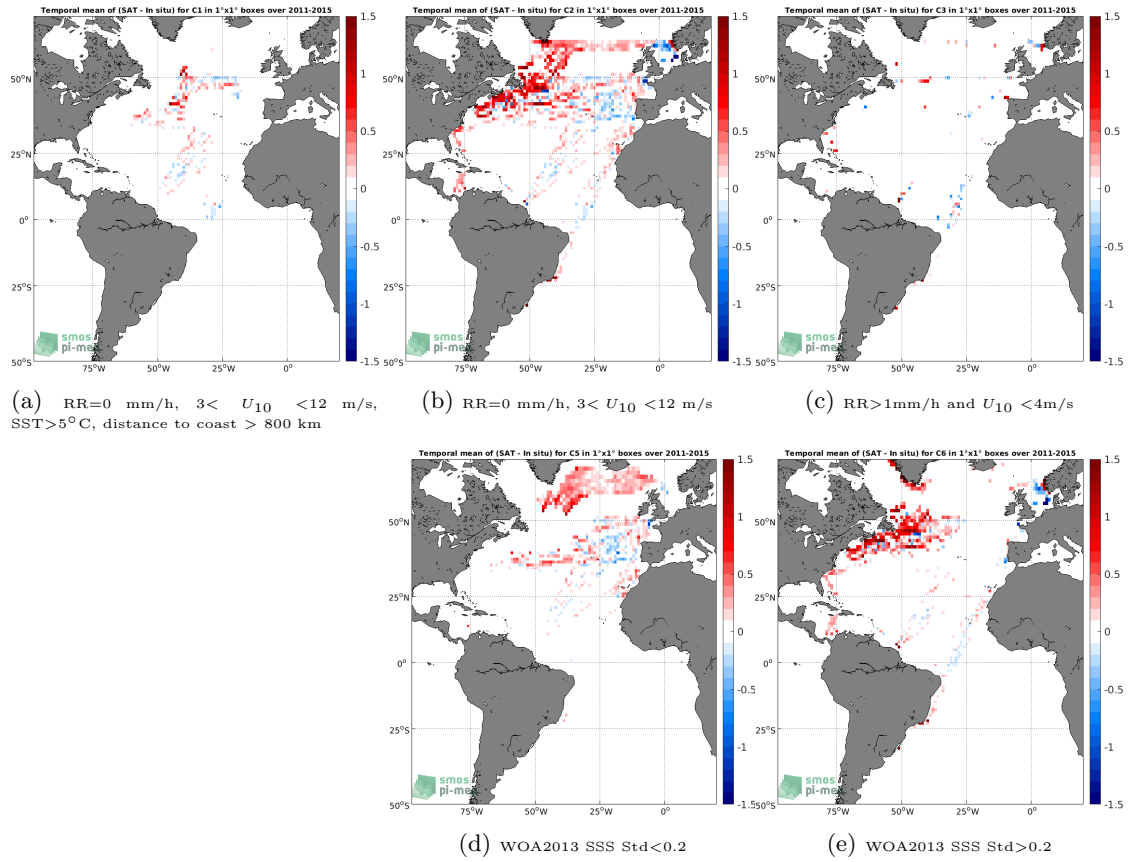
Figure 12: Temporal mean gridded over spatial boxes of size 1^\circ \times 1^\circ of \Delta SSS (Aquarius SSS L3 CAP v5 - 7-Day running (JPL) - TSG (LEGOS-DM)) for 5 different subdatasets corresponding to:RR=0 mm/h, 3 < U_{10} < 12 m/s, SST>5°C, distance to coast > 800 km (a), RR=0 mm/h, 3 < U_{10} < 12 m/s (b), RR>1mm/h and U_{10} < 4 m/s (c), WOA2013 SSS Std<0.2 (d), WOA2013 SSS Std>0.2 (e).
