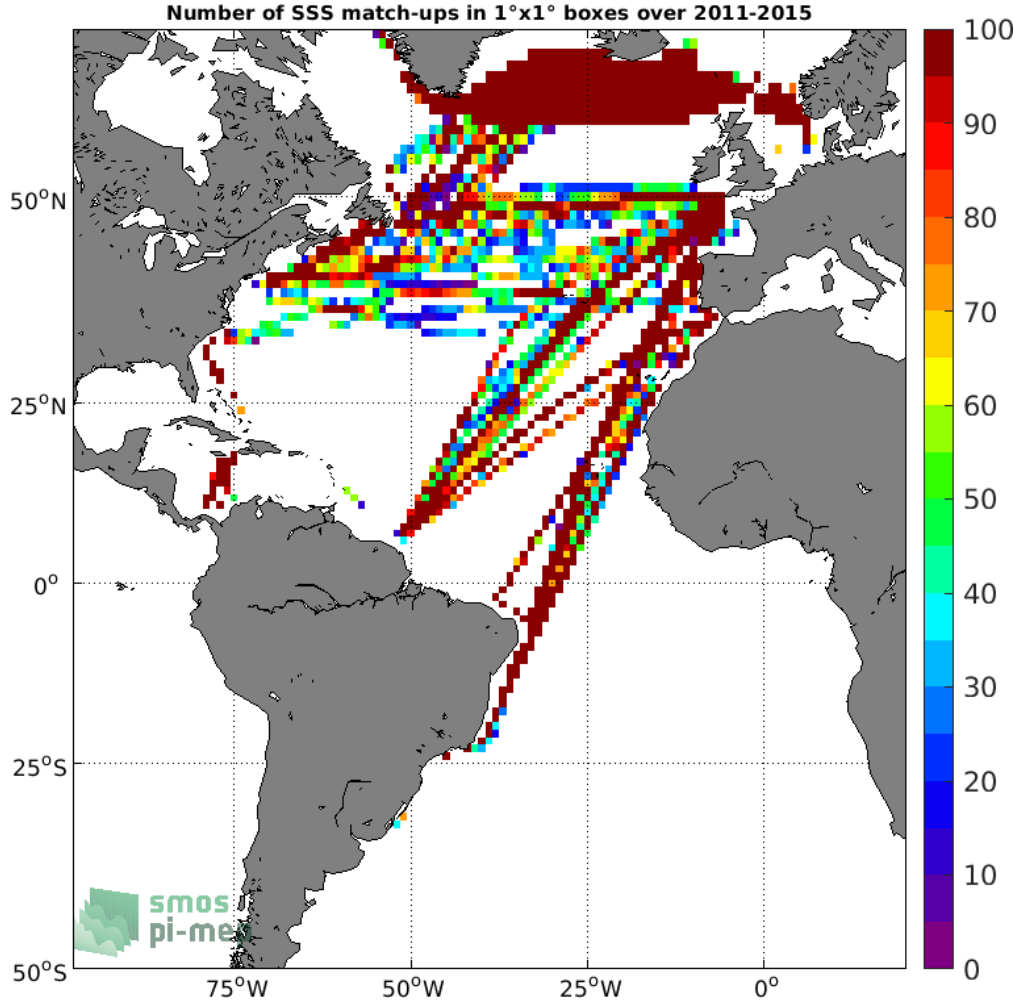
Figure 4: Number of SSS match-ups between TSG (LEGOS-DM) SSS and the Aquarius SSS L3 CAP v5 - 7-Day running (JPL) SSS product for the Atlantic Ocean Pi-MEP region over 1^\circ \times 1^\circ boxes and for the full satellite product period.
