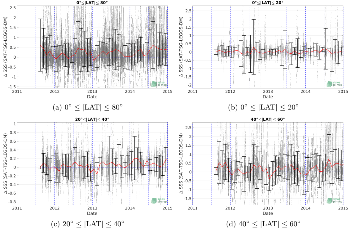
Figure 10: Monthly-averaged mean (red curves) \Delta SSS (Satellite - TSG-LEGOS-DM) and \pm 1 Std (black vertical thick bars) as function of time for all the collected Pi-MEP match-up pairs estimated over the Atlantic Ocean Pi-MEP region and for the full satellite product period are shown for different latitude bands: (a) Latitude band 80^\circ\text{S}-80^\circ\text{N} , (b) latitude band 20^\circ\text{S}-20^\circ\text{N} , (c) Mid Latitude bands 40^\circ\text{S}-20^\circ\text{S} and 20^\circ\text{N}-40^\circ\text{N} and (d) Latitude bands 60^\circ\text{S}-40^\circ\text{S} and 40^\circ\text{N}-60^\circ\text{N} .
