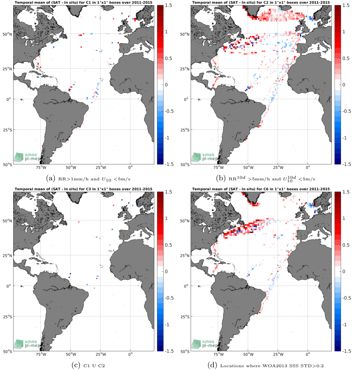
Figure 12: Temporal mean gridded over spatial boxes of size 1^\circ \times 1^\circ of \Delta SSS (Aquarius-L3-JPL-V5-7DAY-RUNNING - TSG-LEGOS-DM) for 4 different subdatasets corresponding to:RR>1mm/h and U_{10} < 5\text{m/s} (a), RR^{10d} > 5\text{mm/h} and U_{10}^{10d} < 5\text{m/s} (b), C1 U C2 (c),Locations where WOA2013 SSS STD>0.2 (d).
