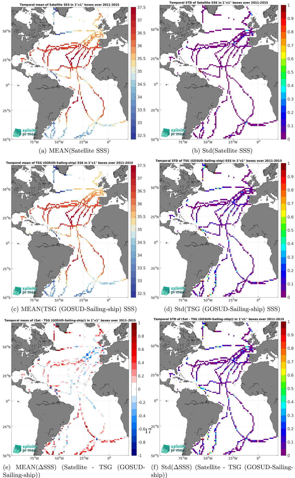
Figure 7: Temporal mean (left) and Std (right) of SSS from Aquarius SSS L3 CAP v5 - 7-Day running (JPL) (top), TSG (GOSUD-Sailing-ship) (middle), and of \Delta SSS (Satellite - TSG (GOSUD-Sailing-ship)). Only match-up pairs are used to generate these maps.
