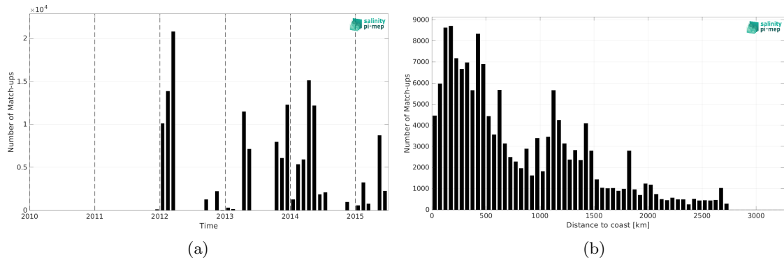
Figure 2: Number of match-ups between TSG (GOSUD-Sailing-ship) and Aquarius SSS L3 CAP v5 - 7-Day running (JPL) SSS as a function of time (a) and as function of the distance to coast (b) over the Atlantic Ocean Pi-MEP region and for the full satellite product period.
