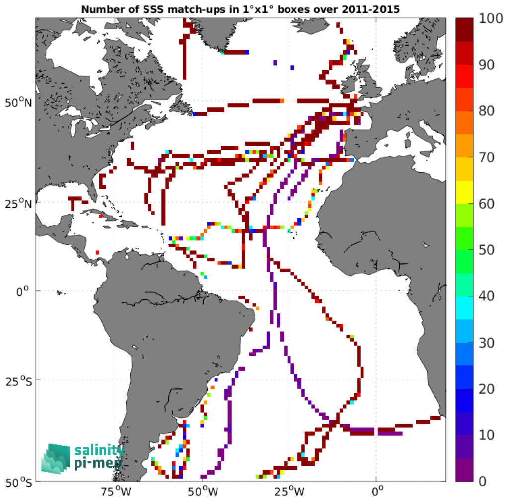
Figure 5: Number of SSS match-ups between TSG (GOSUD-Sailing-ship) SSS and the Aquarius SSS L3 CAP v5 - 7-Day running (JPL) SSS product for the Atlantic Ocean Pi-MEP region over 1^\circ \times 1^\circ boxes and for the full satellite product period.
