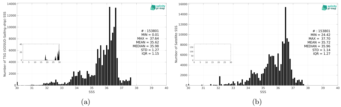
Figure 3: Histograms of SSS from TSG (GOSUD-Sailing-ship) (a) and Aquarius SSS L3 CAP v5 - 7-Day running (JPL) (b) considering all match-up pairs per bins of 0.1 over the Atlantic Ocean Pi-MEP region and for the full satellite product period.
