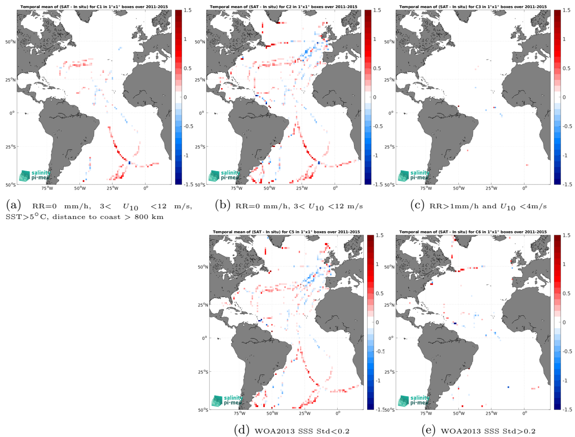
Figure 12: Temporal mean gridded over spatial boxes of size 1^\circ \times 1^\circ of \Delta\text{SSS} (Aquarius SSS L3 CAP v5 - 7-Day running (JPL) - TSG (GOSUD-Sailing-ship)) for 5 different subdatasets corresponding to:RR=0 mm/h, 3 < U_{10} < 12 m/s, SST>5°C, distance to coast > 800 km (a), RR=0 mm/h, 3 < U_{10} < 12 m/s (b), RR>1mm/h and U_{10} < 4 m/s (c), WOA2013 SSS Std<0.2 (d), WOA2013 SSS Std>0.2 (e).
