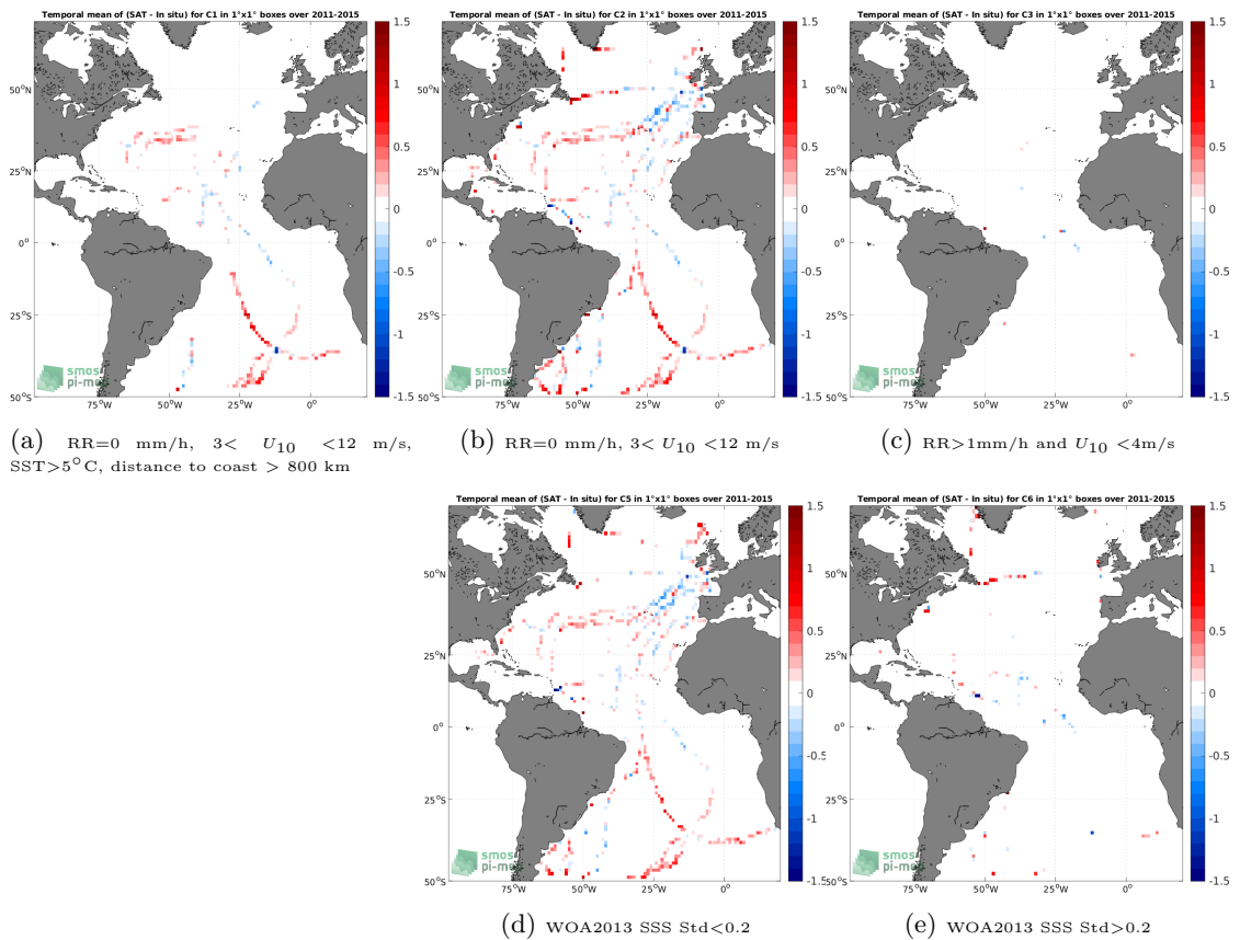
Figure 12: Temporal mean gridded over spatial boxes of size 1^\circ \times 1^\circ of \Delta\text{SSS} (Aquarius SSS L3 CAP v5 - 7-Day running (JPL) - TSG (GOSUD-Sailing-ship)) for 5 different subdatasets corresponding to:RR=0 mm/h, 3 < U_{10} < 12 m/s, SST>5°C, distance to coast > 800 km (a), RR=0 mm/h, 3 < U_{10} < 12 m/s (b), RR>1mm/h and U_{10} < 4 m/s (c), WOA2013 SSS Std<0.2 (d), WOA2013 SSS Std>0.2 (e).
