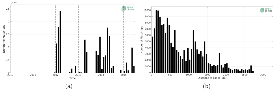
Figure 1: Number of match-ups between TSG (GOSUD-Sailing-ship) and Aquarius SSS L3 CAP v5 - 7-Day running (JPL) SSS as a function of time (a) and as function of the distance to coast (b) over the Atlantic Ocean Pi-MEP region and for the full satellite product period.
