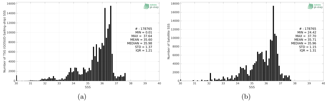
Figure 2: Histograms of SSS from TSG (GOSUD-Sailing-ship) (a) and Aquarius SSS L3 CAP v5 - 7-Day running (JPL) (b) considering all match-up pairs per bins of 0.1 over the Atlantic Ocean Pi-MEP region and for the full satellite product period.
