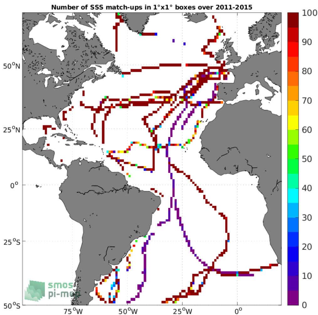
Figure 4: Number of SSS match-ups between TSG (GOSUD-Sailing-ship) SSS and the Aquarius SSS L3 CAP v5 - 7-Day running (JPL) SSS product for the Atlantic Ocean Pi-MEP region over 1°x1° boxes and for the full satellite product period.
