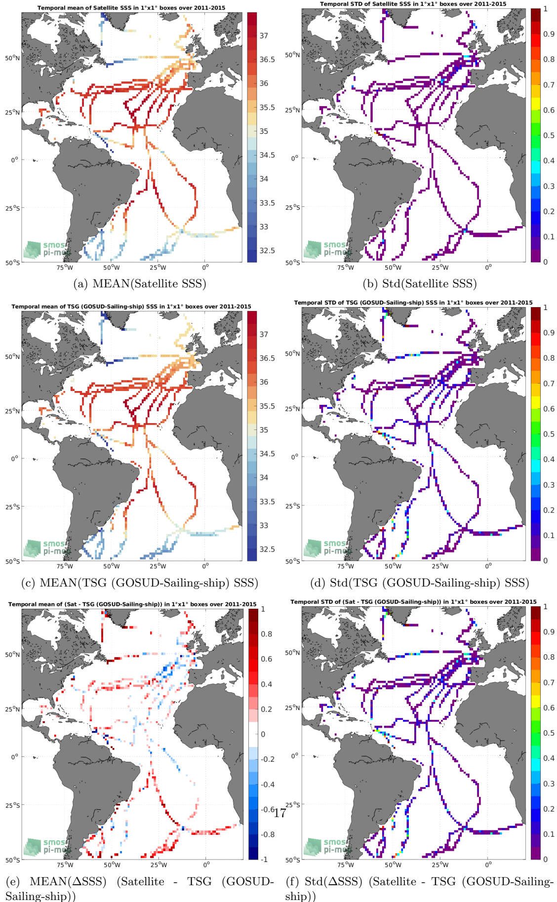
Figure 6: Temporal mean (left) and Std (right) of SSS from Aquarius SSS L3 CAP v5 - 7-Day running (JPL) (top), TSG (GOSUD-Sailing-ship) (middle), and of \Delta SSS (Satellite - TSG (GOSUD-Sailing-ship)). Only match-up pairs are used to generate these maps.
