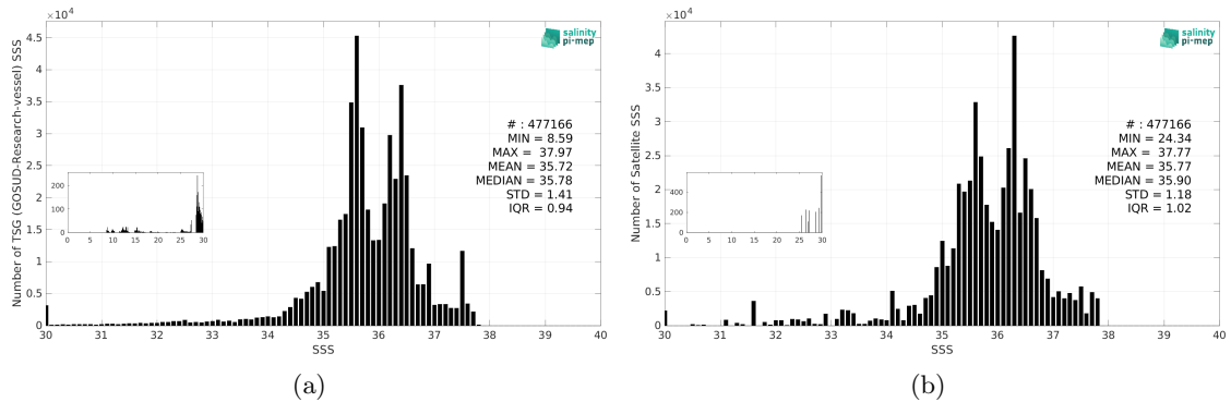
Figure 3: Histograms of SSS from TSG (GOSUD-Research-vessel) (a) and Aquarius SSS L3 CAP v5 - 7-Day running (JPL) (b) considering all match-up pairs per bins of 0.1 over the Atlantic Ocean Pi-MEP region and for the full satellite product period.
