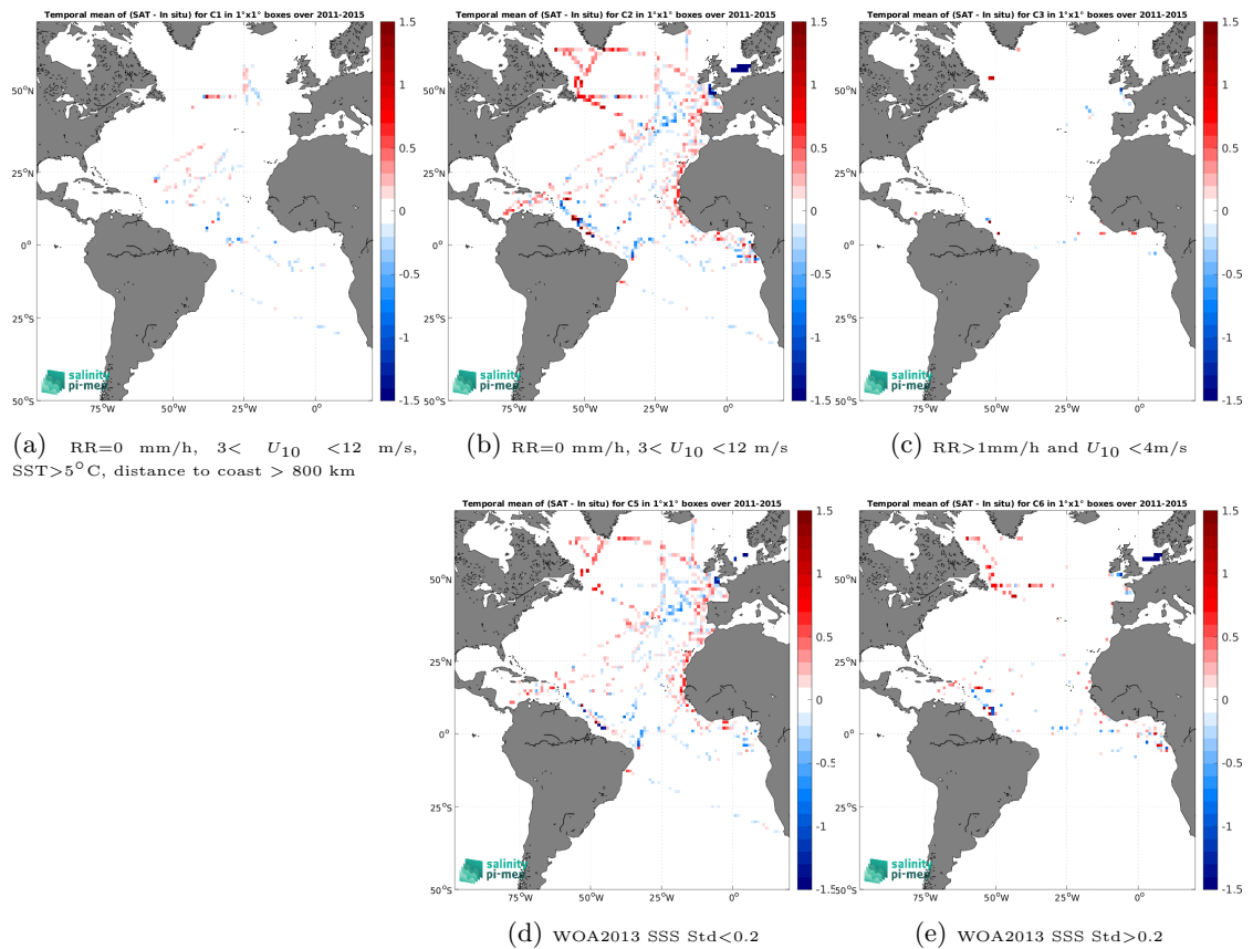
Figure 14: Temporal mean gridded over spatial boxes of size 1^\circ \times 1^\circ of \Delta\text{SSS} (Aquarius SSS L3 CAP v5 - 7-Day running (JPL) - TSG (GOSUD-Research-vessel)) for 5 different subdatasets corresponding to:RR=0 mm/h, 3 < U_{10} < 12 m/s, SST>5°C, distance to coast > 800 km (a), RR=0 mm/h, 3 < U_{10} < 12 m/s (b), RR>1mm/h and U_{10} < 4 m/s (c), WOA2013 SSS Std<0.2 (d), WOA2013 SSS Std>0.2 (e).
