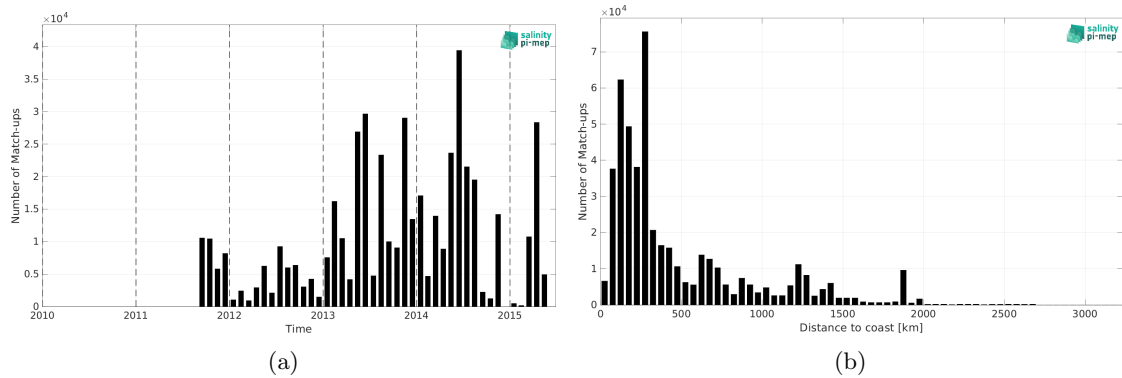
Figure 2: Number of match-ups between TSG (GOSUD-Research-vessel) and Aquarius SSS L3 CAP v5 - 7-Day running (JPL) SSS as a function of time (a) and as function of the distance to coast (b) over the Atlantic Ocean Pi-MEP region and for the full satellite product period.
