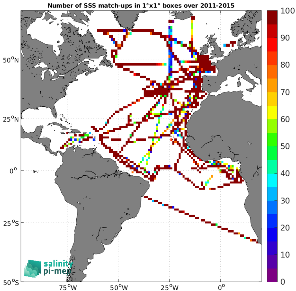
Figure 5: Number of SSS match-ups between TSG (GOSUD-Research-vessel) SSS and the Aquarius SSS L3 CAP v5 - 7-Day running (JPL) SSS product for the Atlantic Ocean Pi-MEP region over 1^\circ \times 1^\circ boxes and for the full satellite product period.
