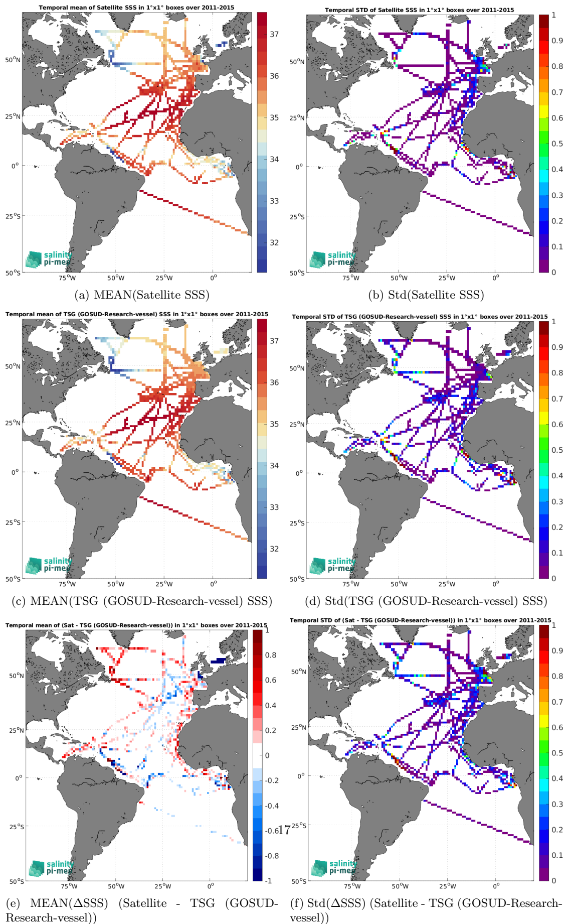
Figure 7: Temporal mean (left) and Std (right) of SSS from Aquarius SSS L3 CAP v5 - 7-Day running (JPL) (top), TSG (GOSUD-Research-vessel) (middle), and of \Delta SSS (Satellite - TSG (GOSUD-Research-vessel)). Only match-up pairs are used to generate these maps.
