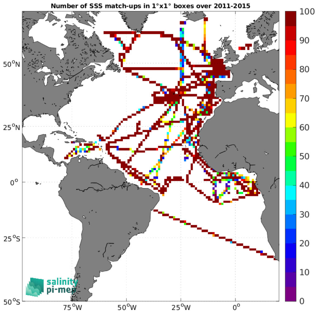
Figure 4: Number of SSS match-ups between TSG (GOSUD-Research-vessel) SSS and the Aquarius SSS L3 CAP v5 - 7-Day running (JPL) SSS product for the Atlantic Ocean Pi-MEP region over 1^{\circ} \times 1^{\circ} boxes and for the full satellite product period.
