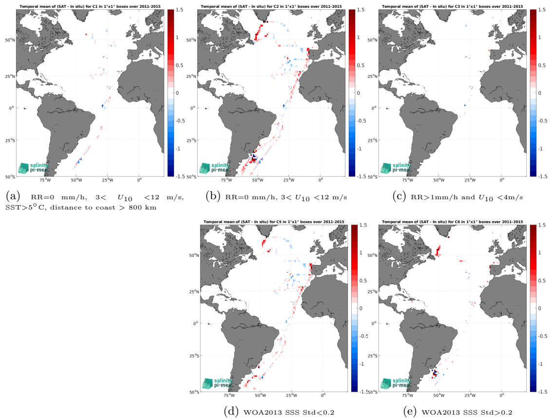
Figure 14: Temporal mean gridded over spatial boxes of size 1^\circ \times 1^\circ of \Delta SSS (Aquarius SSS L3 CAP v5 - 7-Day running (JPL) - TSG (CSIC-UTM)) for 5 different subdatasets corresponding to:RR=0 mm/h, 3 < U_{10} < 12 m/s, SST >5^\circ\text{C} , distance to coast > 800 km (a), RR=0 mm/h, 3 < U_{10} < 12 m/s (b), RR >1 mm/h and U_{10} < 4 m/s (c), WOA2013 SSS Std <0.2 (d), WOA2013 SSS Std >0.2 (e).
