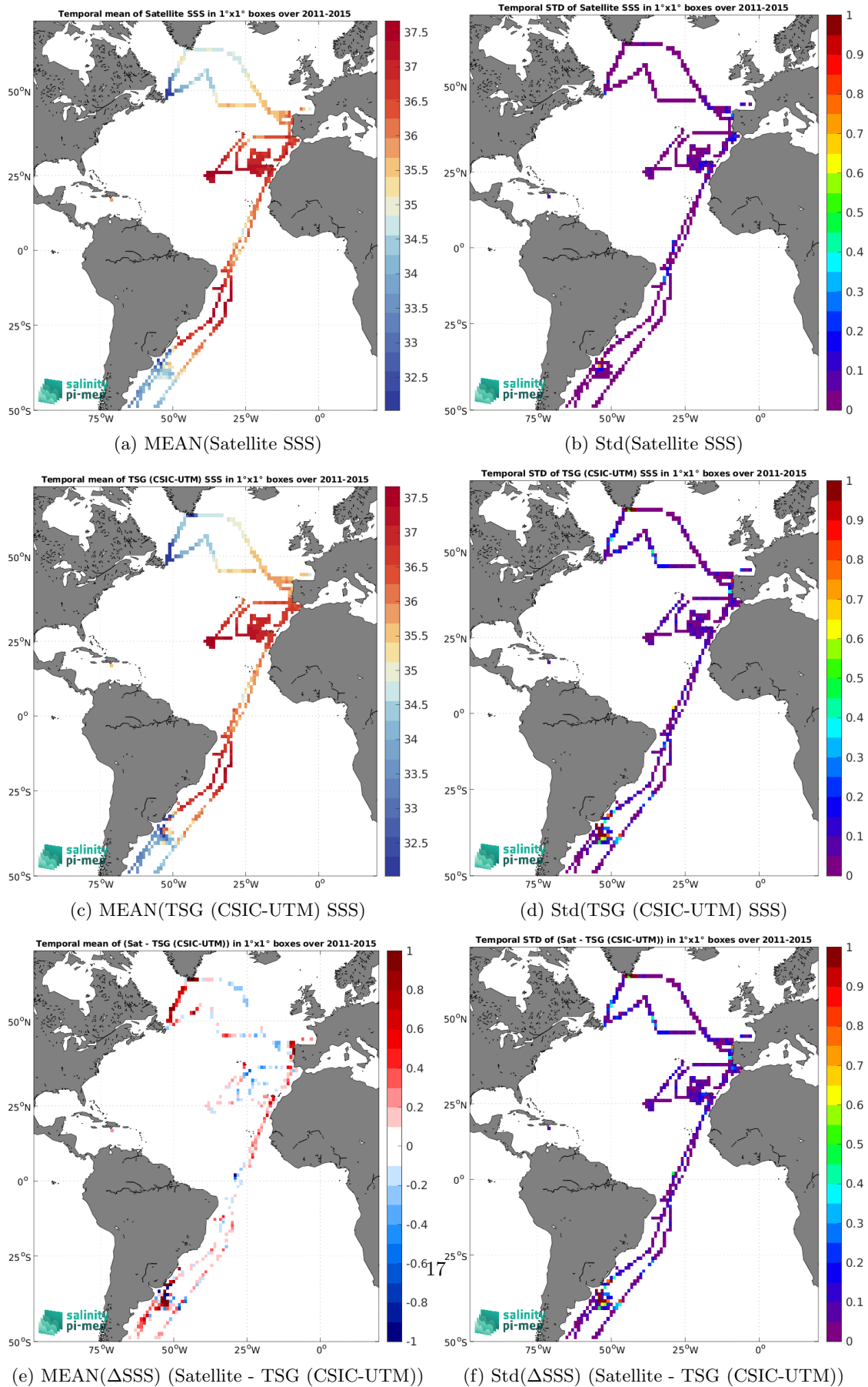
Figure 7: Temporal mean (left) and Std (right) of SSS from Aquarius SSS L3 CAP v5 - 7-Day running (JPL) (top), TSG (CSIC-UTM) (middle), and of \Delta SSS (Satellite - TSG (CSIC-UTM)). Only match-up pairs are used to generate these maps.
