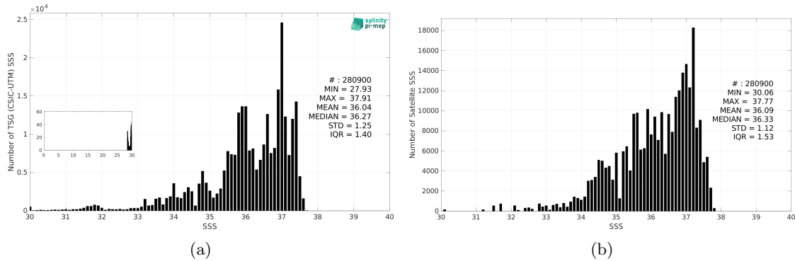
Figure 3: Histograms of SSS from TSG (CSIC-UTM) (a) and Aquarius SSS L3 CAP v5 - 7-Day running (JPL) (b) considering all match-up pairs per bins of 0.1 over the Atlantic Ocean Pi-MEP region and for the full satellite product period.
