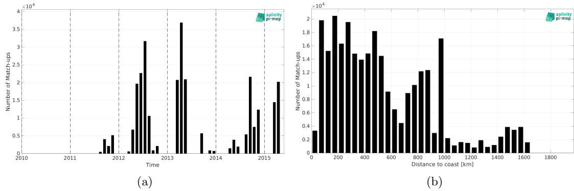
Figure 2: Number of match-ups between TSG (CSIC-UTM) and Aquarius SSS L3 CAP v5 - 7-Day running (JPL) SSS as a function of time (a) and as function of the distance to coast (b) over the Atlantic Ocean Pi-MEP region and for the full satellite product period.
