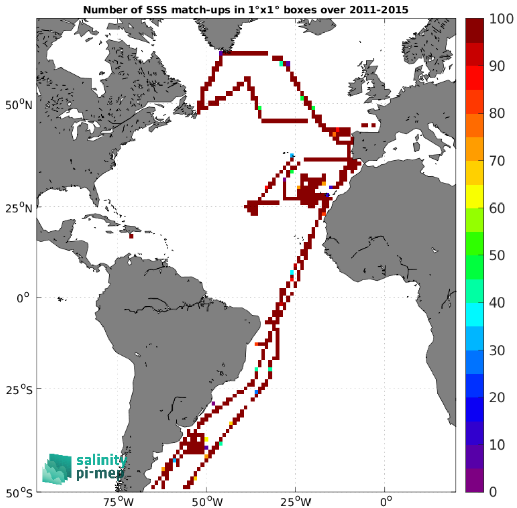
Figure 5: Number of SSS match-ups between TSG (CSIC-UTM) SSS and the Aquarius SSS L3 CAP v5 - 7-Day running (JPL) SSS product for the Atlantic Ocean Pi-MEP region over 1^\circ \times 1^\circ boxes and for the full satellite product period.
