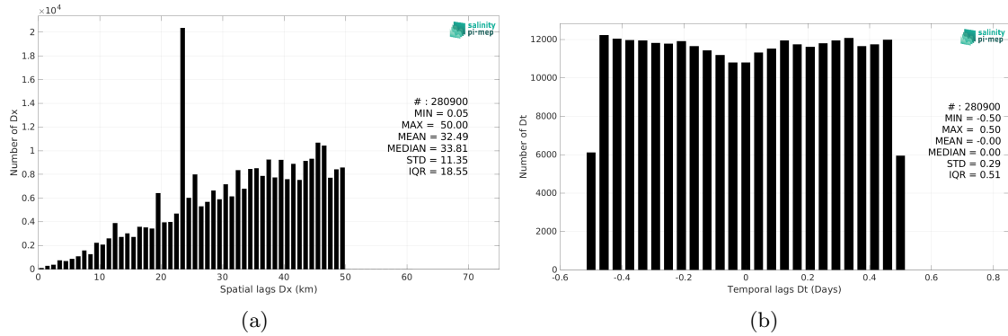
Figure 6: Histograms of the spatial (a) and temporal (b) lags between the location/time of the TSG (CSIC-UTM) measurement and the date of the corresponding Aquarius SSS L3 CAP v5 - 7-Day running (JPL) SSS pixel.
