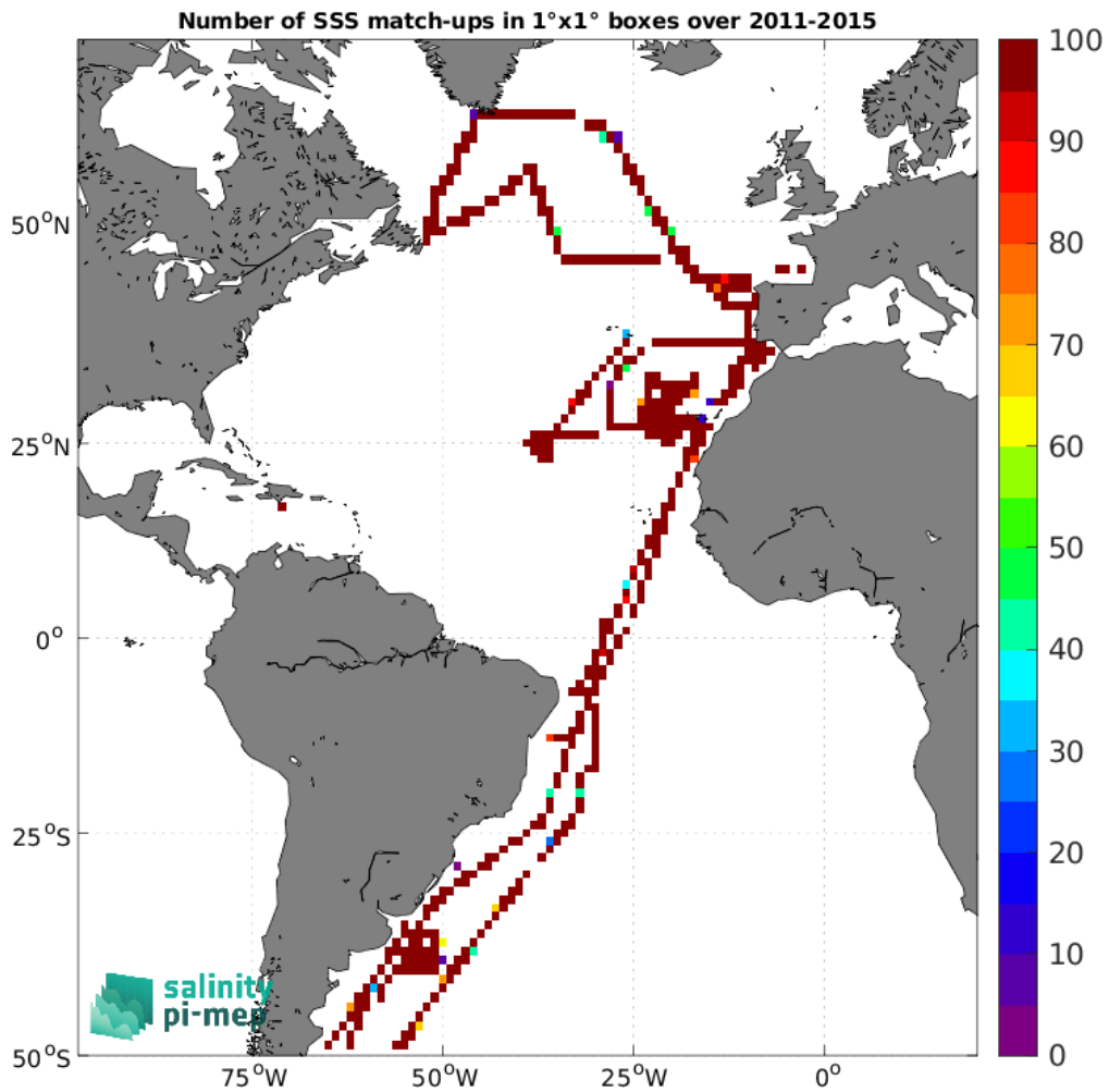
Figure 5: Number of SSS match-ups between TSG (CSIC-UTM) SSS and the Aquarius SSS L3 CAP v5 - 7-Day running (JPL) SSS product for the Atlantic Ocean Pi-MEP region over 1°x1° boxes and for the full satellite product period.
