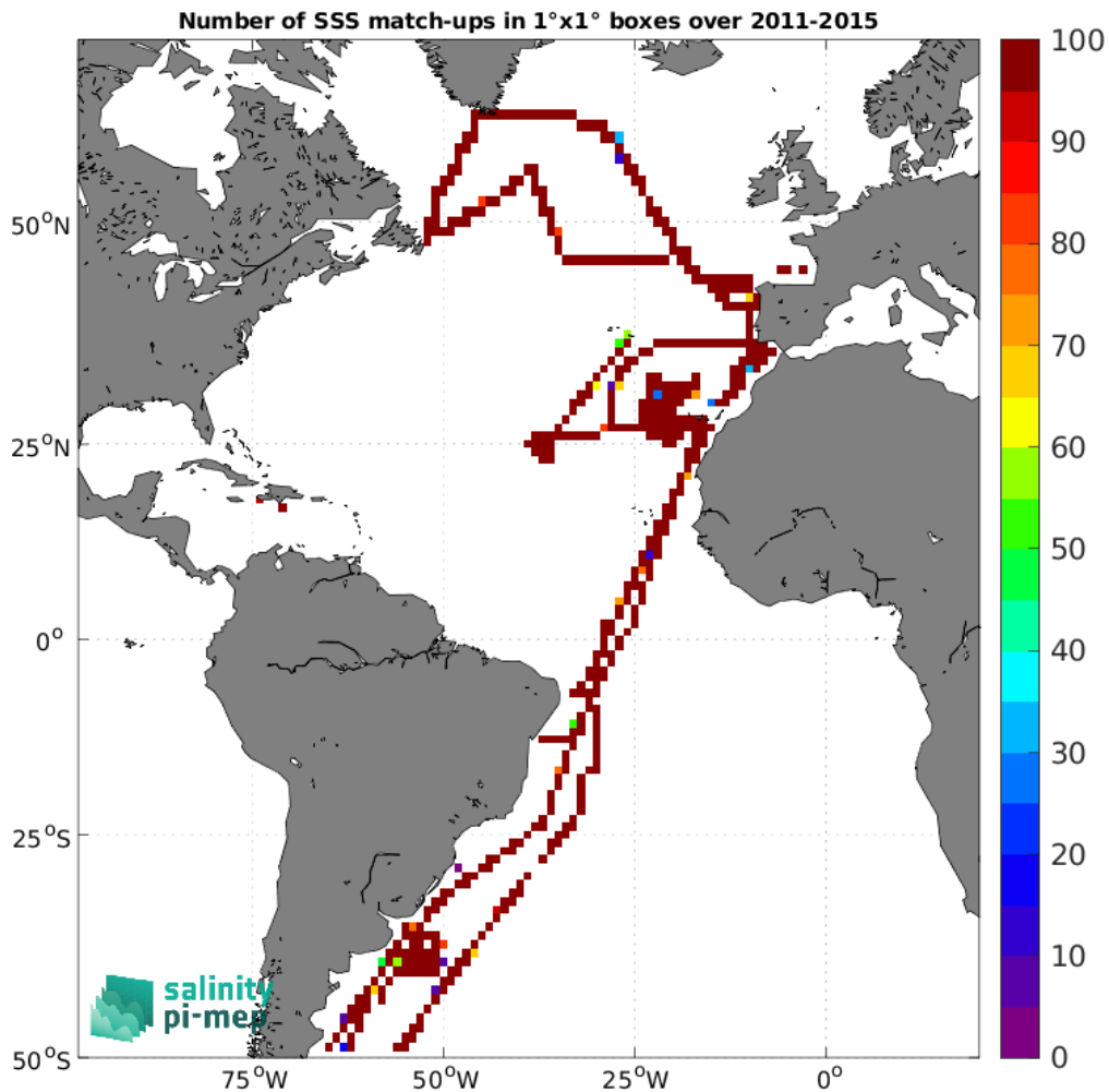
Figure 4: Number of SSS match-ups between TSG (CSIC-UTM) SSS and the Aquarius SSS L3 CAP v5 - 7-Day running (JPL) SSS product for the Atlantic Ocean Pi-MEP region over 1°x1° boxes and for the full satellite product period.
