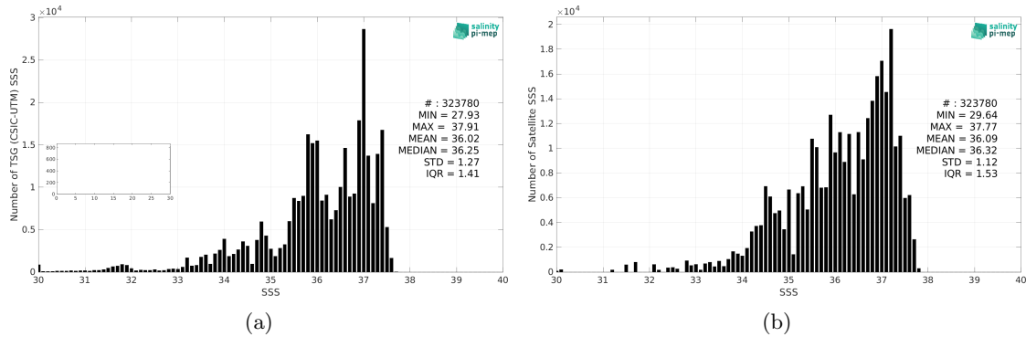
Figure 2: Histograms of SSS from TSG (CSIC-UTM) (a) and Aquarius SSS L3 CAP v5 - 7-Day running (JPL) (b) considering all match-up pairs per bins of 0.1 over the Atlantic Ocean Pi-MEP region and for the full satellite product period.
