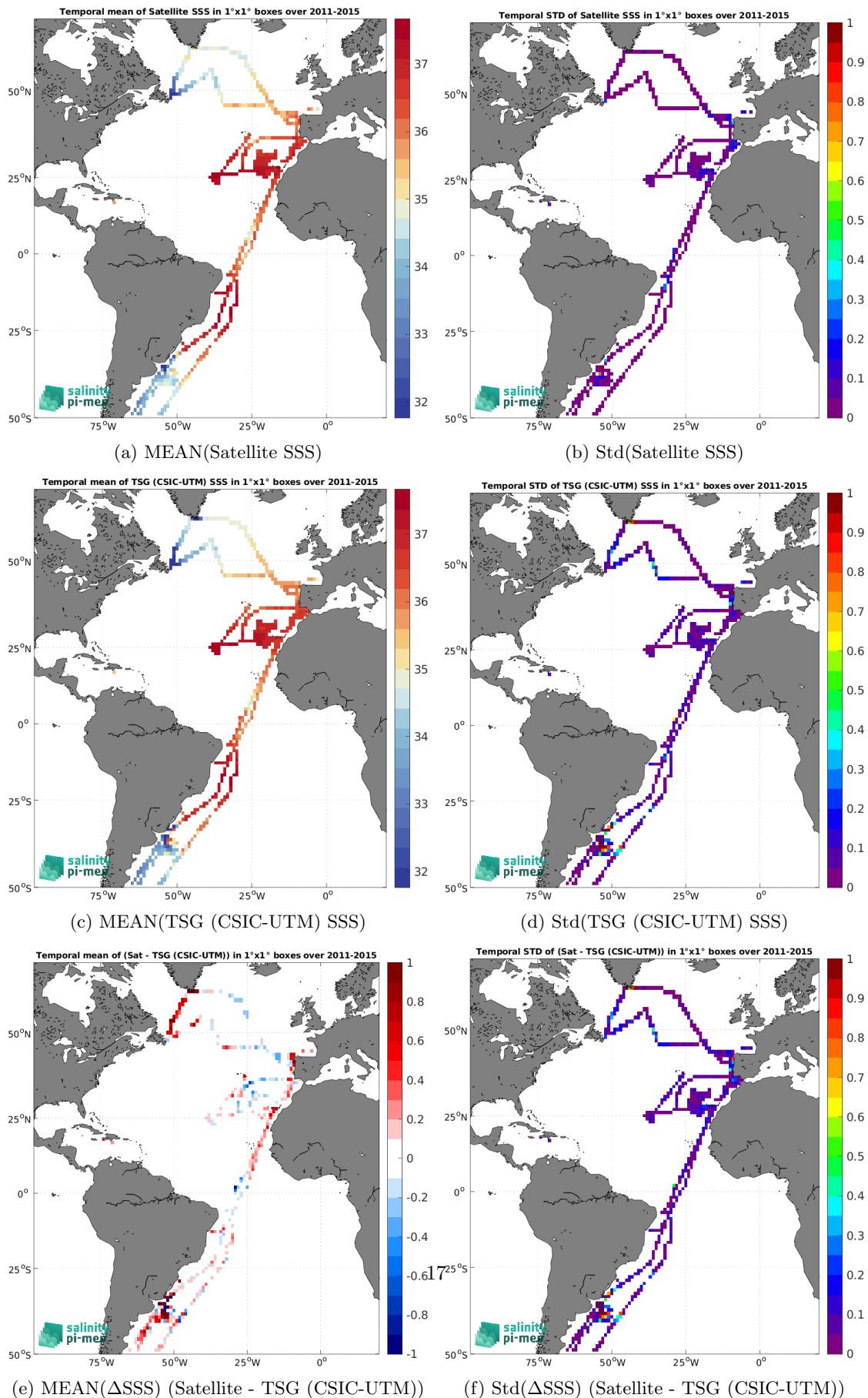
Figure 6: Temporal mean (left) and Std (right) of SSS from Aquarius SSS L3 CAP v5 - 7-Day running (JPL) (top), TSG (CSIC-UTM) (middle), and of \Delta SSS (Satellite - TSG (CSIC-UTM)). Only match-up pairs are used to generate these maps.
