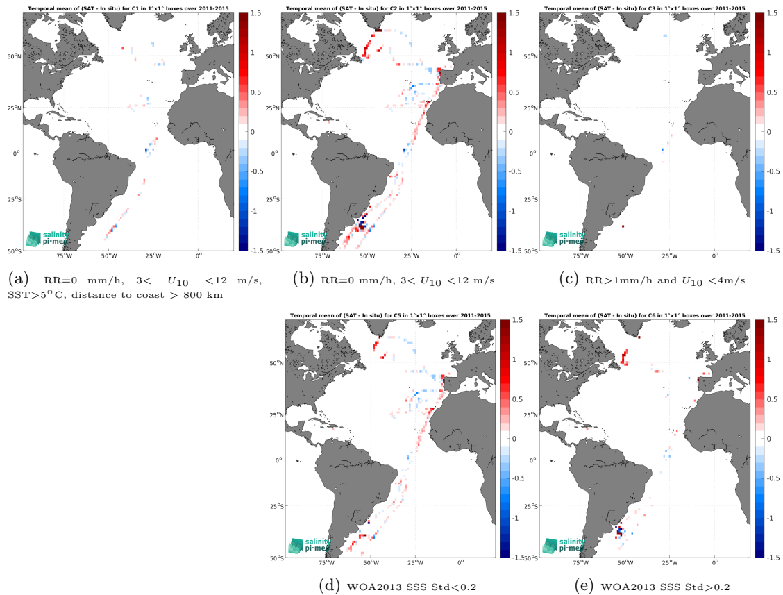
Figure 12: Temporal mean gridded over spatial boxes of size 1^\circ \times 1^\circ of \Delta SSS (Aquarius SSS L3 CAP v5 - 7-Day running (JPL) - TSG (CSIC-UTM)) for 5 different subdatasets corresponding to:RR=0 mm/h, 3 < U_{10} < 12 m/s, SST >5^\circ\text{C} , distance to coast > 800 km (a), RR=0 mm/h, 3 < U_{10} < 12 m/s (b), RR >1 mm/h and U_{10} < 4 m/s (c), WOA2013 SSS Std <0.2 (d), WOA2013 SSS Std >0.2 (e).
