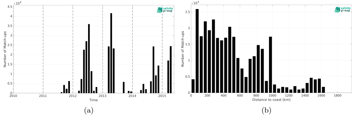
Figure 1: Number of match-ups between TSG (CSIC-UTM) and Aquarius SSS L3 CAP v5 - 7-Day running (JPL) SSS as a function of time (a) and as function of the distance to coast (b) over the Atlantic Ocean Pi-MEP region and for the full satellite product period.
