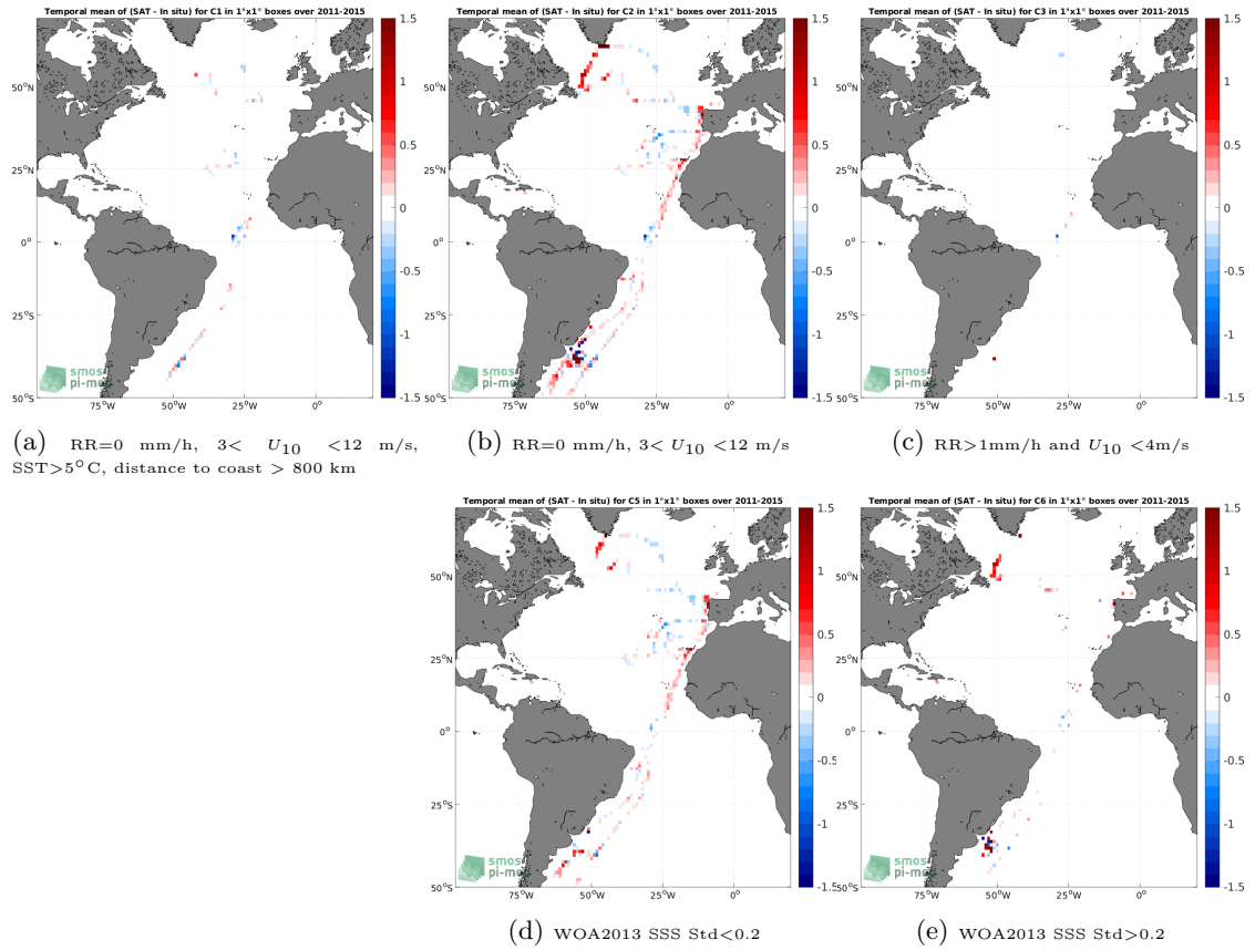
Figure 12: Temporal mean gridded over spatial boxes of size 1^\circ \times 1^\circ of \Delta SSS (Aquarius SSS L3 CAP v5 - 7-Day running (JPL) - TSG (CSIC-UTM)) for 5 different subdatasets corresponding to:RR=0 mm/h, 3 < U_{10} < 12 m/s, SST >5^\circ\text{C} , distance to coast > 800 km (a), RR=0 mm/h, 3 < U_{10} < 12 m/s (b), RR >1 mm/h and U_{10} < 4 m/s (c), WOA2013 SSS Std <0.2 (d), WOA2013 SSS Std >0.2 (e).
