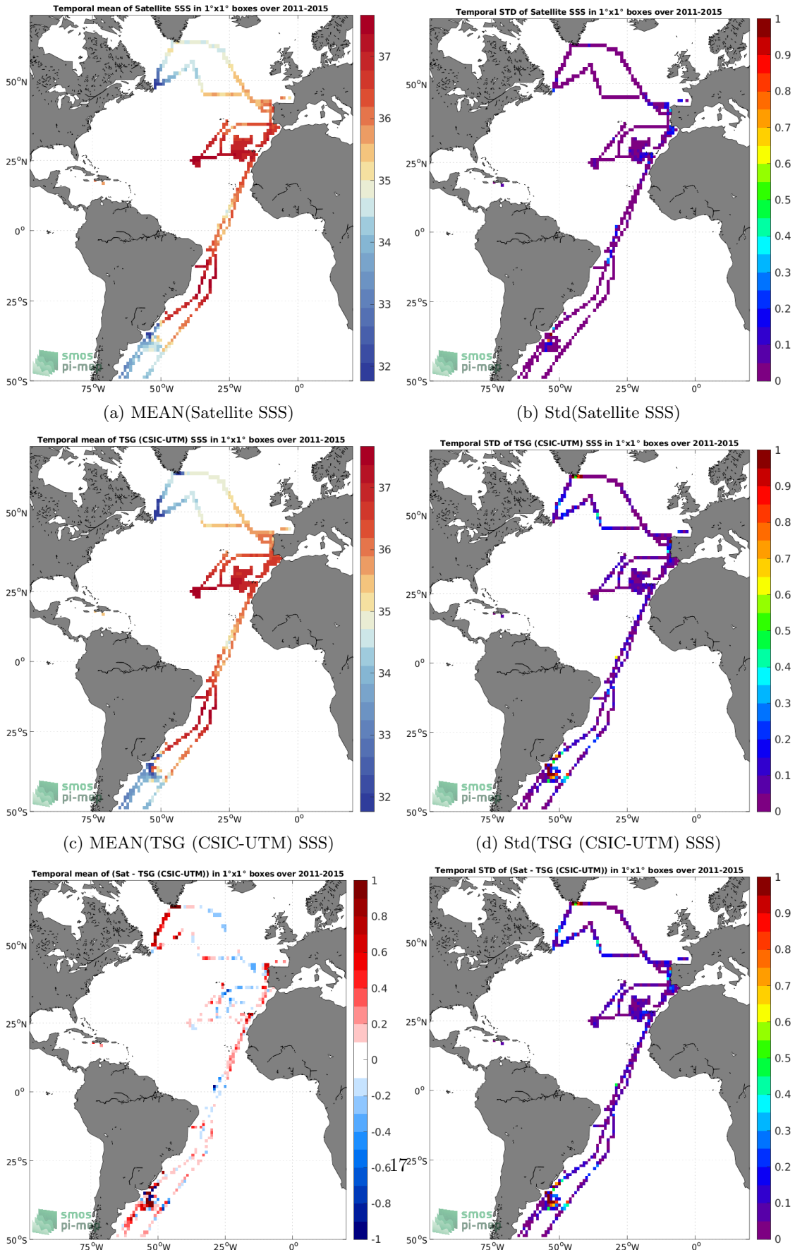
(e) MEAN( \Delta SSS) (Satellite - TSG (CSIC-UTM)) (f) Std( \Delta SSS) (Satellite - TSG (CSIC-UTM)) Figure 6: Temporal mean (left) and Std (right) of SSS from Aquarius SSS L3 CAP v5 - 7-Day running (JPL) (top), TSG (CSIC-UTM) (middle), and of \Delta SSS (Satellite - TSG (CSIC-UTM)). Only match-up pairs are used to generate these maps.
