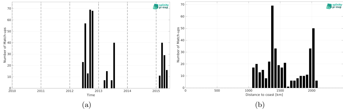
Figure 1: Number of match-ups between Marine mammals and Aquarius SSS L3 CAP v5 - 7-Day running (JPL) SSS as a function of time (a) and as function of the distance to coast (b) over the Atlantic Ocean Pi-MEP region and for the full satellite product period.
