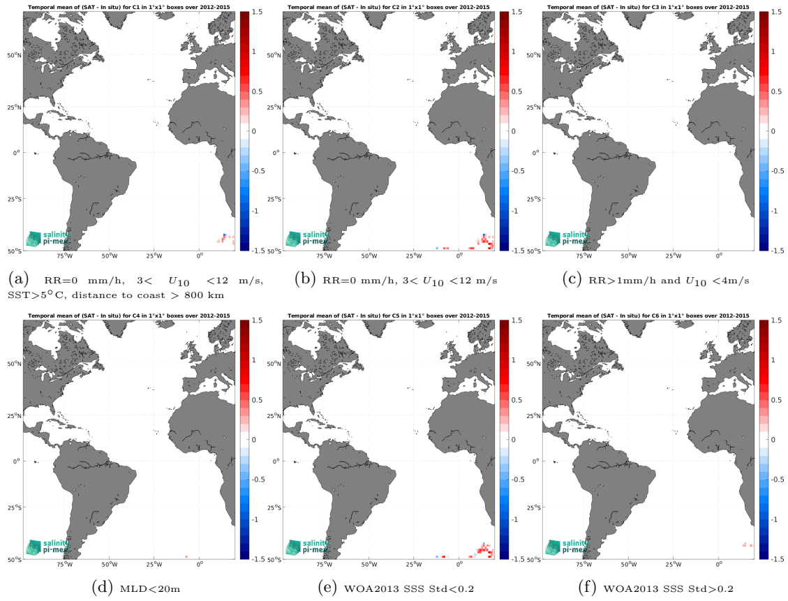
Figure 12: Temporal mean gridded over spatial boxes of size 1^\circ \times 1^\circ of \Delta SSS (Aquarius SSS L3 CAP v5 - 7-Day running (JPL) - Marine mammals) for 6 different subdatasets corresponding to: RR=0 mm/h, 3 < U_{10} < 12 m/s, SST > 5°C, distance to coast > 800 km (a), RR=0 mm/h, 3 < U_{10} < 12 m/s (b), RR > 1mm/h and U_{10} < 4 m/s (c), MLD < 20m (d), WOA2013 SSS Std < 0.2 (e), WOA2013 SSS Std > 0.2 (f).
