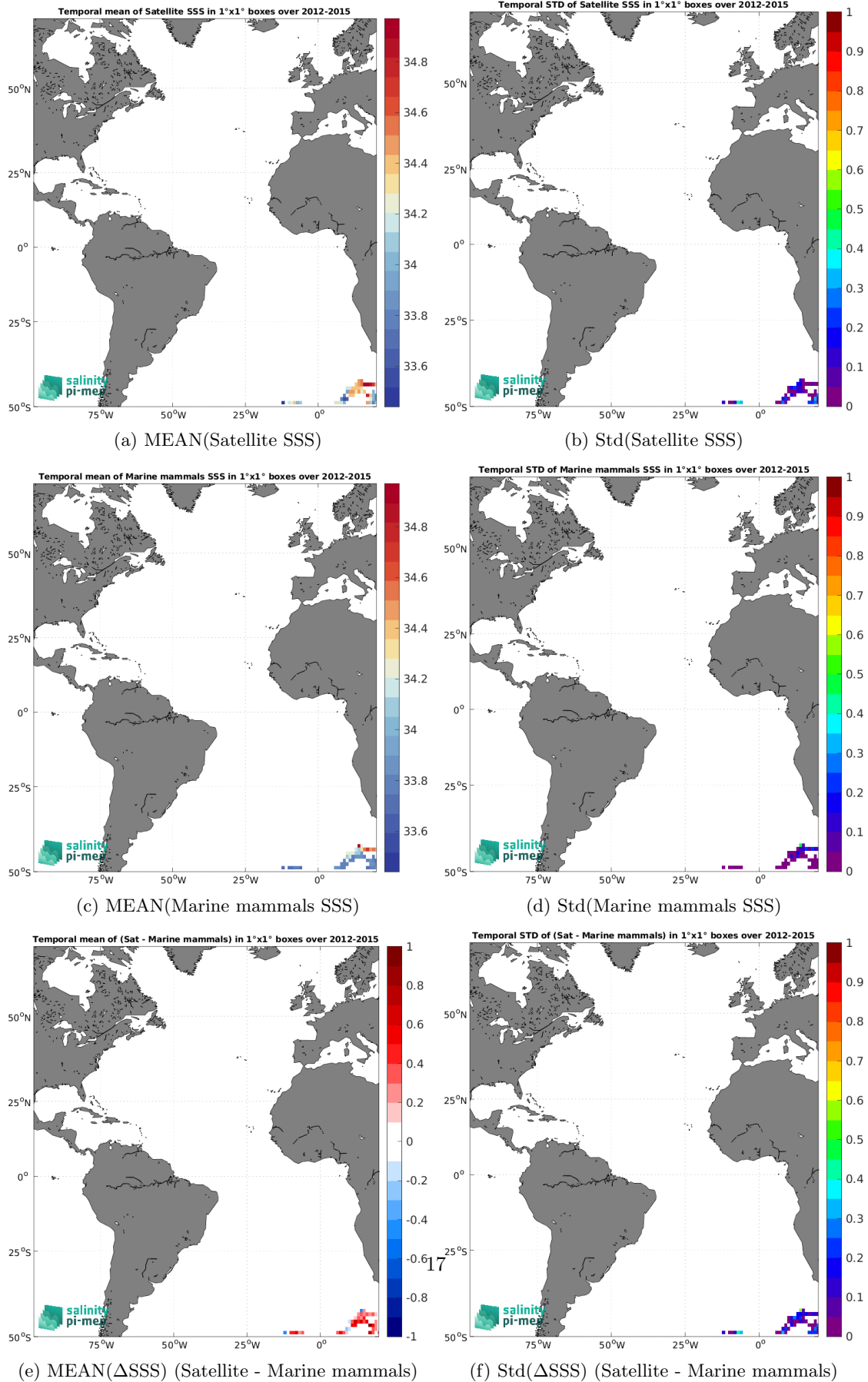
Figure 6: Temporal mean (left) and Std (right) of SSS from Aquarius SSS L3 CAP v5 - 7-Day running (JPL) (top), Marine mammals (middle), and of \Delta SSS (Satellite - Marine mammals). Only match-up pairs are used to generate these maps.
