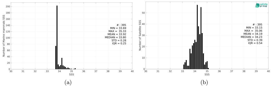
Figure 2: Histograms of SSS from Marine mammals (a) and Aquarius SSS L3 CAP v5 - 7-Day running (JPL) (b) considering all match-up pairs per bins of 0.1 over the Atlantic Ocean Pi-MEP region and for the full satellite product period.
