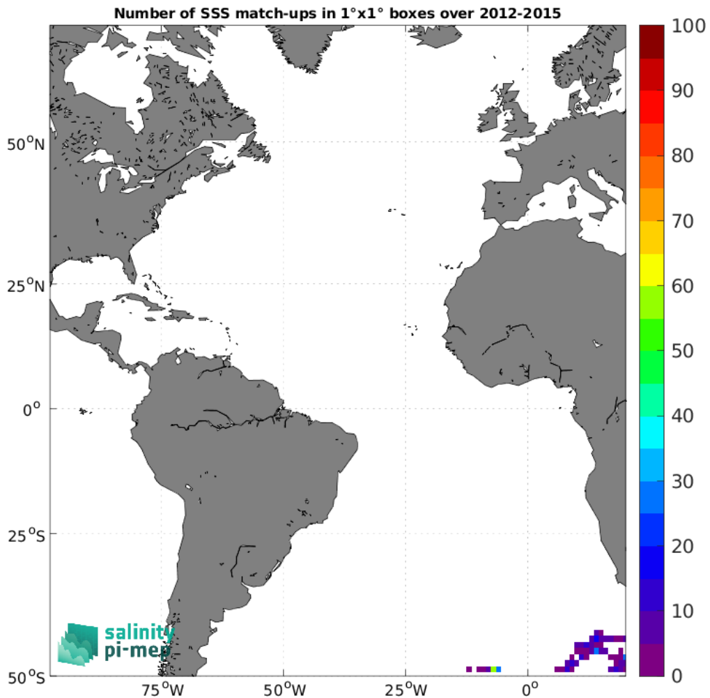
Figure 4: Number of SSS match-ups between Marine mammals SSS and the Aquarius SSS L3 CAP v5 - 7-Day running (JPL) SSS product for the Atlantic Ocean Pi-MEP region over 1^\circ \times 1^\circ boxes and for the full satellite product period.
