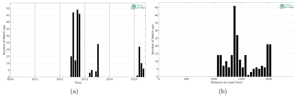
Figure 1: Number of match-ups between Sea mammals and Aquarius-L3-JPL-V5-7DAY-RUNNING SSS as a function of time (a) and as function of the distance to coast (b) over the Atlantic Ocean Pi-MEP region and for the full satellite product period.
