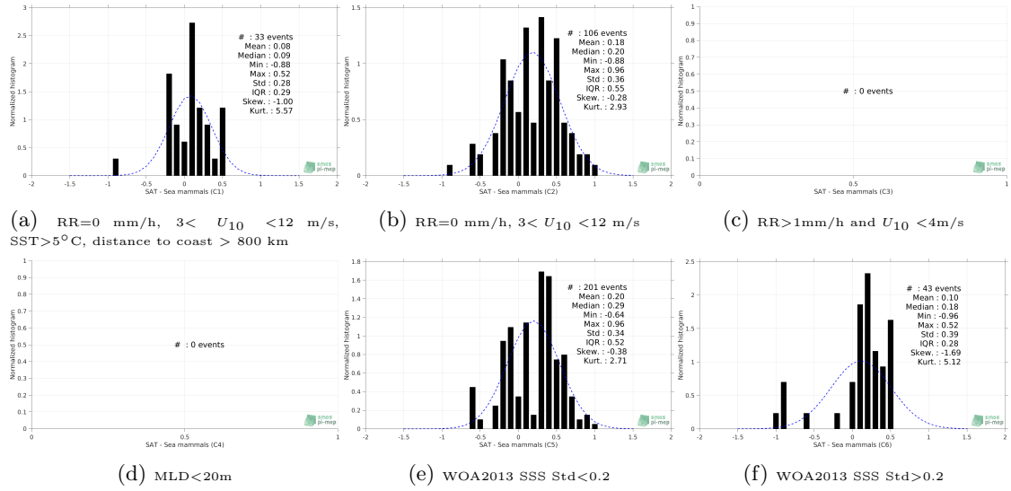
Figure 13: Normalized histogram of \Delta SSS (Aquarius-L3-JPL-V5-7DAY-RUNNING - Sea mammals) for 6 different subdatasets corresponding to: RR=0 mm/h, 3 < U_{10} < 12 m/s, SST>5°C, distance to coast > 800 km (a), RR=0 mm/h, 3 < U_{10} < 12 m/s (b), RR>1mm/h and U_{10} < 4 m/s (c), MLD<20m (d), WOA2013 SSS Std<0.2 (e), WOA2013 SSS Std>0.2 (f).
