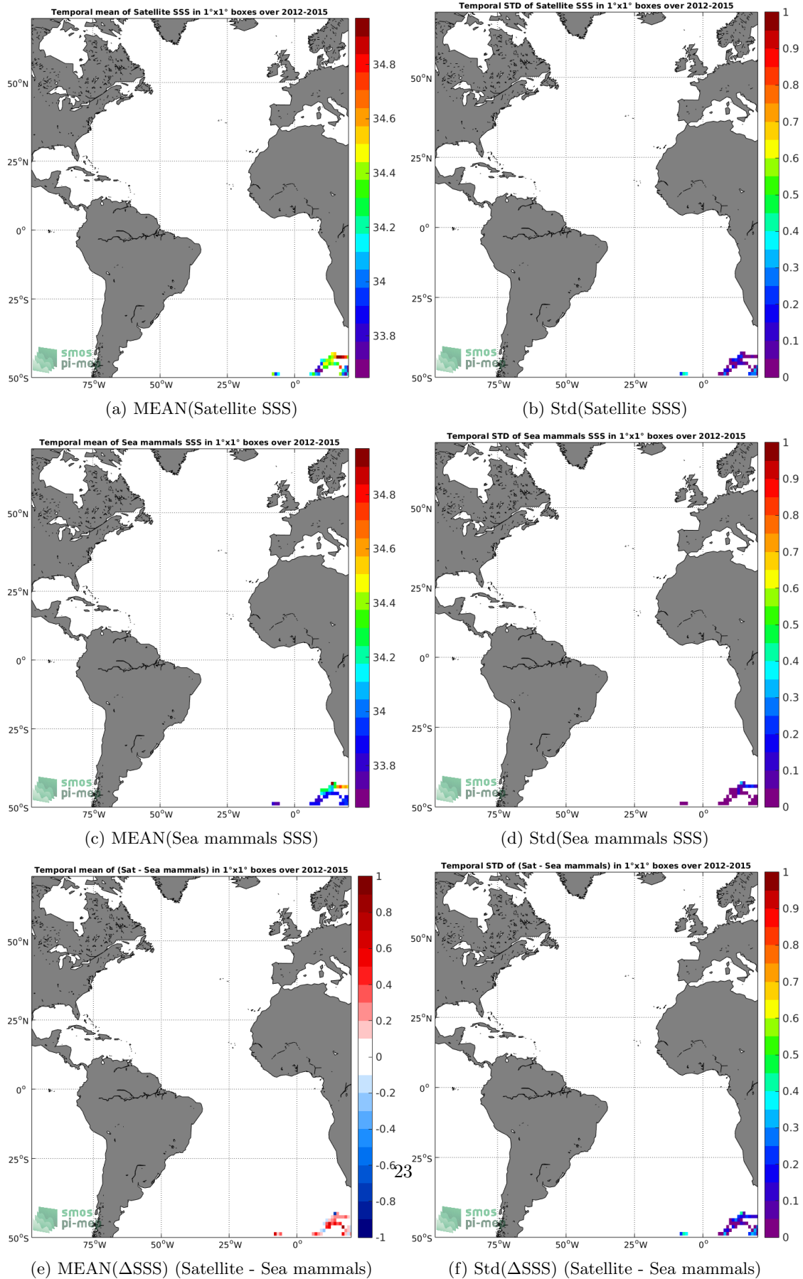
Figure 6: Temporal mean (left) and Std (right) of SSS from Aquarius-L3-JPL-V5-7DAY-RUNNING (top), Sea mammals (middle), and of \Delta SSS (Satellite - Sea mammals). Only match-up pairs are used to generate these maps.
