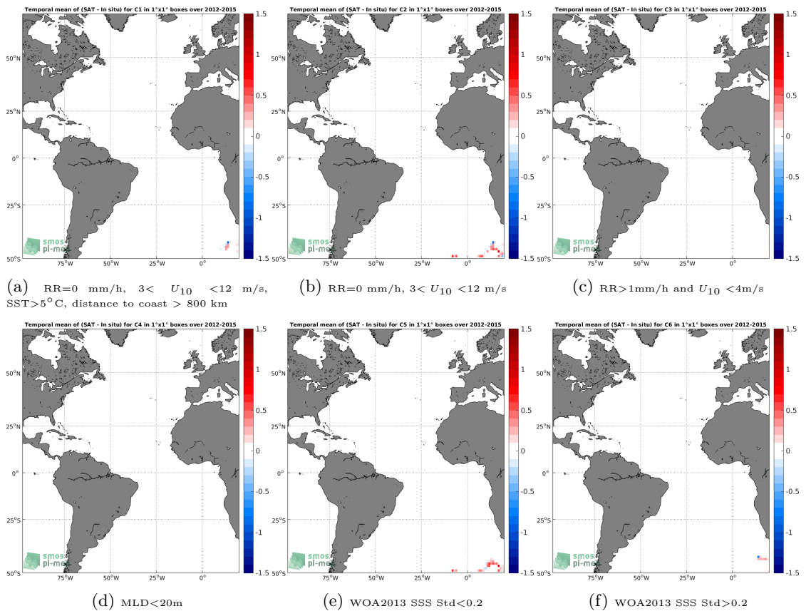
Figure 12: Temporal mean gridded over spatial boxes of size 1°x1° of \Delta SSS (Aquarius-L3-JPL-V5-7DAY-RUNNING - Sea mammals) for 6 different subdatasets corresponding to:RR=0 mm/h, 3 < U_{10} < 12 m/s, SST>5°C, distance to coast > 800 km (a), RR=0 mm/h, 3 < U_{10} < 12 m/s (b), RR>1mm/h and U_{10} < 4 m/s (c),MLD<20m (d),WOA2013 SSS Std<0.2 (e),WOA2013 SSS Std>0.2 (f).
