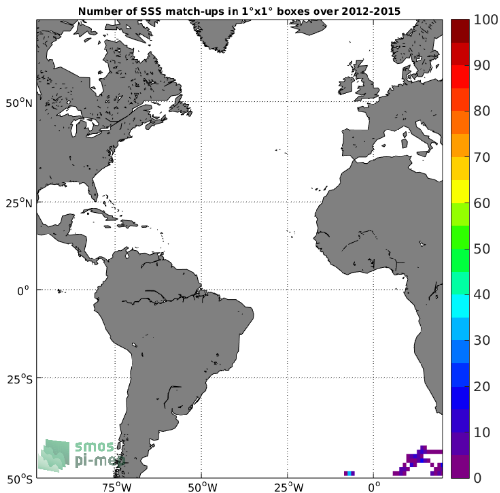
Figure 4: Number of SSS match-ups between Sea mammals SSS and the Aquarius-L3-JPL-V5-7DAY-RUNNING SSS product for the Atlantic Ocean Pi-MEP region over 1°x1° boxes and for the full satellite product period.
