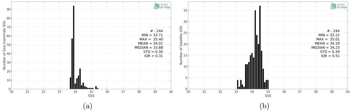
Figure 2: Histograms of SSS from Sea mammals (a) and Aquarius-L3-JPL-V5-7DAY-RUNNING (b) considering all match-up pairs per bins of 0.1 over the Atlantic Ocean Pi-MEP region and for the full satellite product period.
