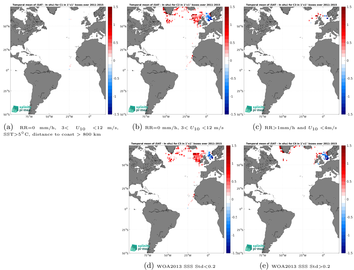
Figure 14: Temporal mean gridded over spatial boxes of size 1^\circ \times 1^\circ of \Delta\text{SSS} (Aquarius SSS L3 CAP v5 - 7-Day running (JPL) - ICES) for 5 different subdatasets corresponding to:RR=0 mm/h, 3 < U_{10} < 12 m/s, SST>5°C, distance to coast > 800 km (a), RR=0 mm/h, 3 < U_{10} < 12 m/s (b), RR>1mm/h and U_{10} < 4 m/s (c), WOA2013 SSS Std<0.2 (d), WOA2013 SSS Std>0.2 (e).
