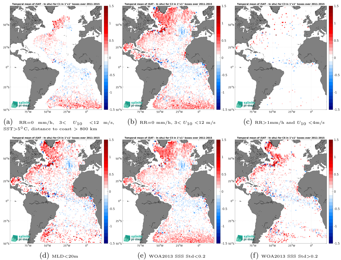
Figure 14: Temporal mean gridded over spatial boxes of size 1^\circ \times 1^\circ of \Delta SSS (Aquarius SSS L3 CAP v5 - 7-Day running (JPL) - Argo) for 6 different subdatasets corresponding to:RR=0 mm/h, 3 < U_{10} < 12 m/s, SST > 5^\circ\text{C} , distance to coast > 800 km (a), RR=0 mm/h, 3 < U_{10} < 12 m/s (b), RR > 1 mm/h and U_{10} < 4 m/s (c),MLD < 20 m (d),WOA2013 SSS Std < 0.2 (e),WOA2013 SSS Std > 0.2 (f).
