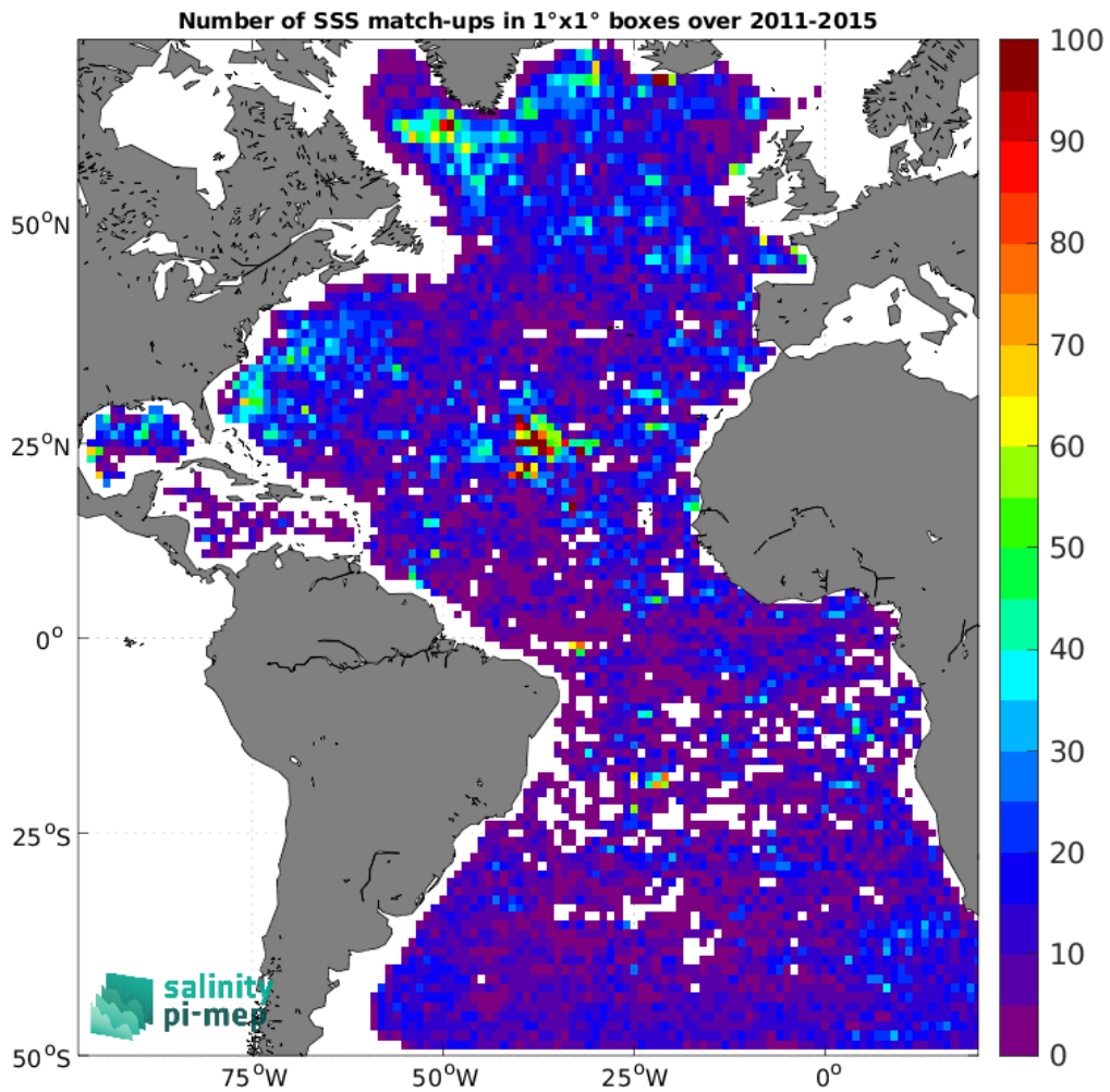
Figure 5: Number of SSS match-ups between Argo SSS and the Aquarius SSS L3 CAP v5 - 7-Day running (JPL) SSS product for the Atlantic Ocean Pi-MEP region over 1^\circ \times 1^\circ boxes and for the full satellite product period.
