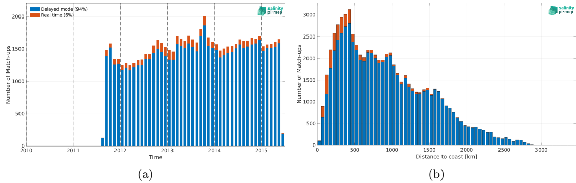
Figure 2: Number of match-ups between Argo and Aquarius SSS L3 CAP v5 - 7-Day running (JPL) SSS as a function of time (a) and as function of the distance to coast (b) over the Atlantic Ocean Pi-MEP region and for the full satellite product period.
