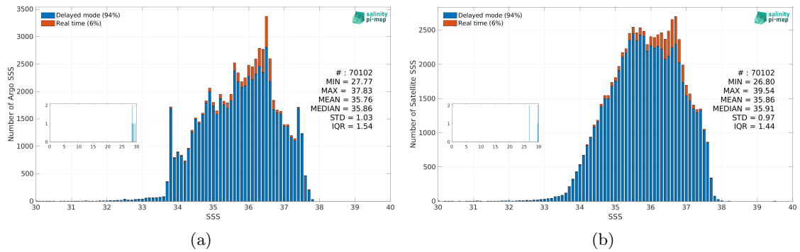
Figure 3: Histograms of SSS from Argo (a) and Aquarius SSS L3 CAP v5 - 7-Day running (JPL) (b) considering all match-up pairs per bins of 0.1 over the Atlantic Ocean Pi-MEP region and for the full satellite product period.
