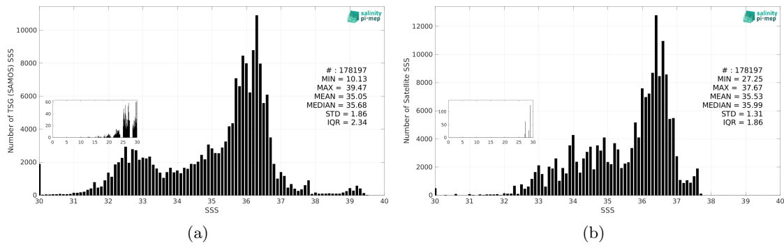
Figure 3: Histograms of SSS from TSG (SAMOS) (a) and Aquarius SSS L3 CAP v5 - Monthly (JPL) (b) considering all match-up pairs per bins of 0.1 over the Atlantic Ocean Pi-MEP region and for the full satellite product period.
