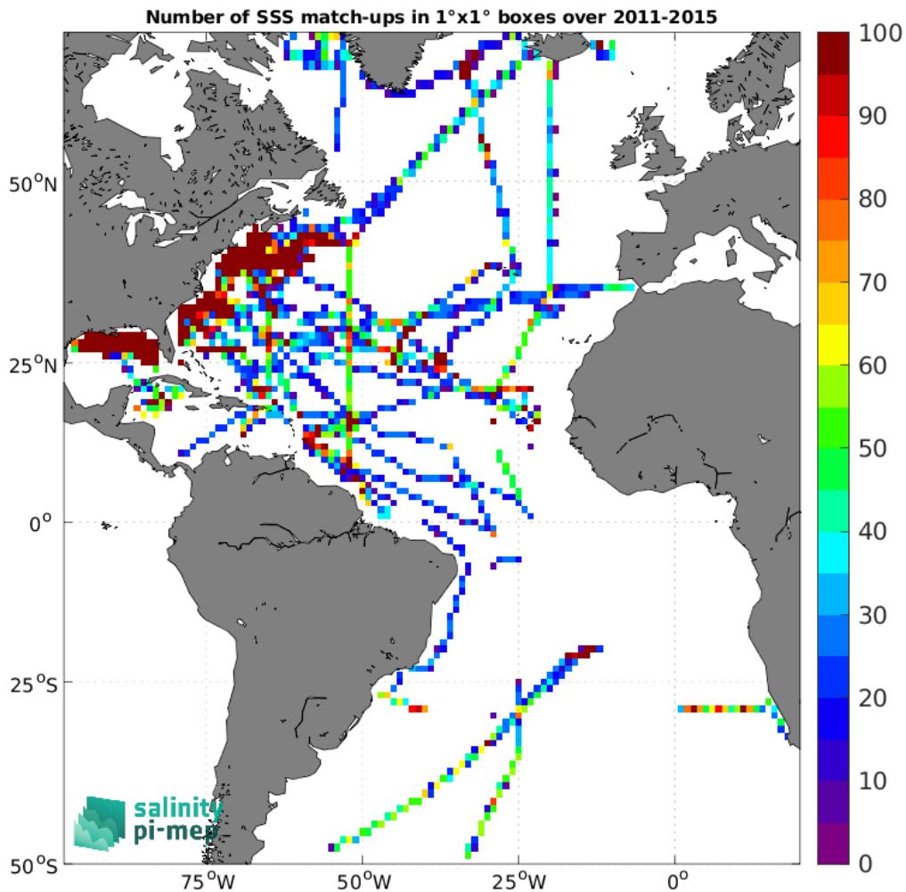
Figure 5: Number of SSS match-ups between TSG (SAMOS) SSS and the Aquarius SSS L3 CAP v5 - Monthly (JPL) SSS product for the Atlantic Ocean Pi-MEP region over 1^\circ \times 1^\circ boxes and for the full satellite product period.
