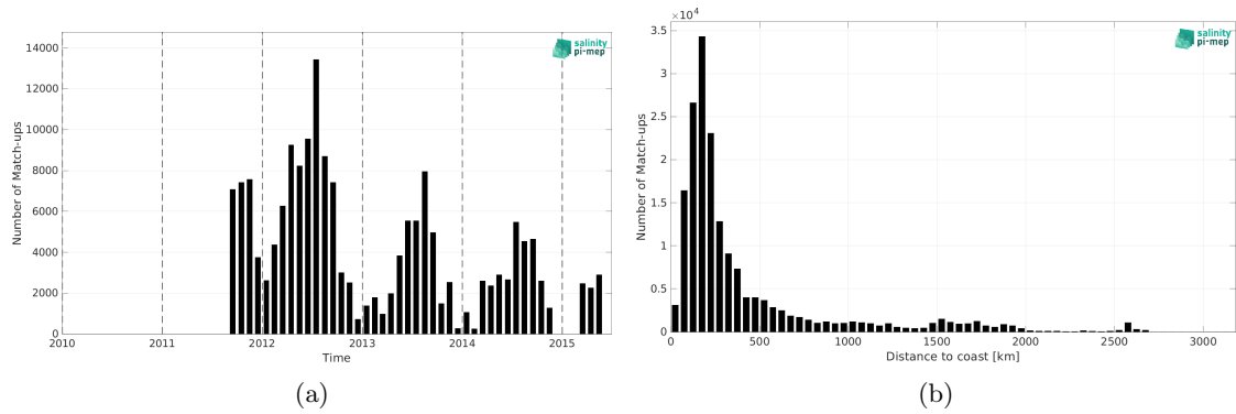
Figure 2: Number of match-ups between TSG (SAMOS) and Aquarius SSS L3 CAP v5 - Monthly (JPL) SSS as a function of time (a) and as function of the distance to coast (b) over the Atlantic Ocean Pi-MEP region and for the full satellite product period.
