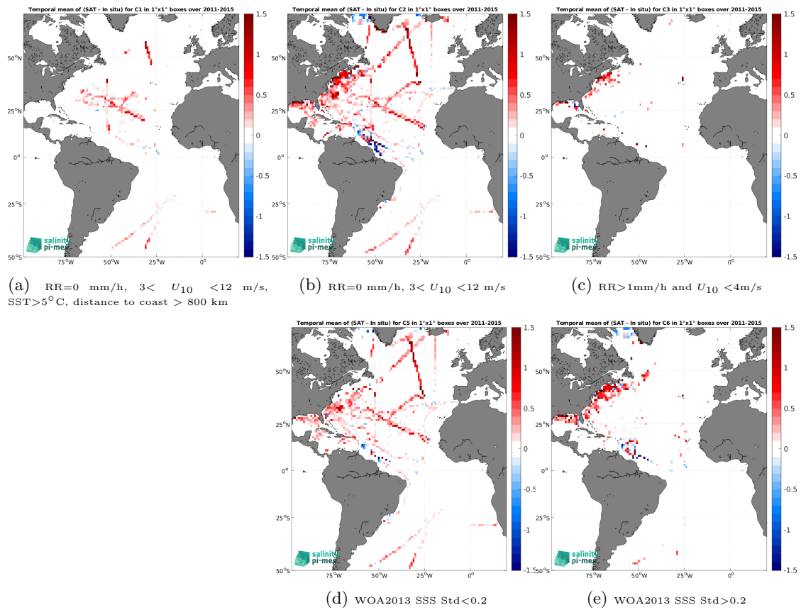
Figure 14: Temporal mean gridded over spatial boxes of size 1^\circ \times 1^\circ of \Delta SSS (Aquarius SSS L3 CAP v5 - Monthly (JPL) - TSG (SAMOS)) for 5 different subdatasets corresponding to:RR=0 mm/h, 3 < U_{10} < 12 m/s, SST >5^\circ\text{C} , distance to coast > 800 km (a), RR=0 mm/h, 3 < U_{10} < 12 m/s (b), RR >1 mm/h and U_{10} < 4 m/s (c), WOA2013 SSS Std <0.2 (d), WOA2013 SSS Std >0.2 (e).
