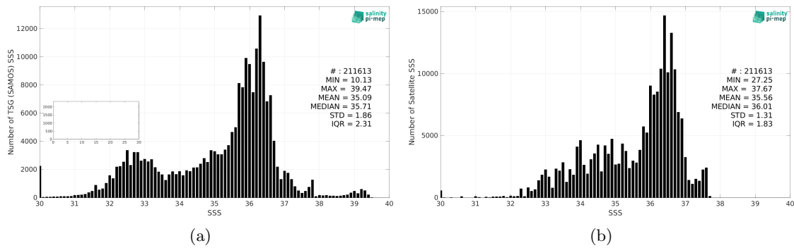
Figure 2: Histograms of SSS from TSG (SAMOS) (a) and Aquarius SSS L3 CAP v5 - Monthly (JPL) (b) considering all match-up pairs per bins of 0.1 over the Atlantic Ocean Pi-MEP region and for the full satellite product period.
