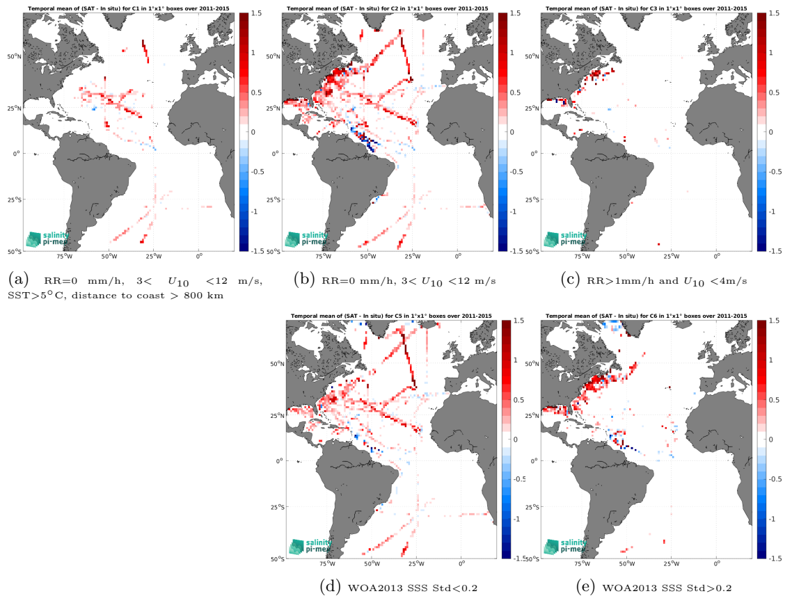
Figure 12: Temporal mean gridded over spatial boxes of size 1^\circ \times 1^\circ of \Delta SSS (Aquarius SSS L3 CAP v5 - Monthly (JPL) - TSG (SAMOS)) for 5 different subdatasets corresponding to:RR=0 mm/h, 3 < U_{10} < 12 m/s, SST >5^\circ\text{C} , distance to coast > 800 km (a), RR=0 mm/h, 3 < U_{10} < 12 m/s (b), RR >1 mm/h and U_{10} < 4 m/s (c), WOA2013 SSS Std <0.2 (d), WOA2013 SSS Std >0.2 (e).
