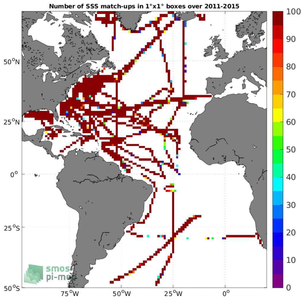
Figure 4: Number of SSS match-ups between TSG (SAMOS) SSS and the Aquarius SSS L3 CAP v5 - Monthly (JPL) SSS product for the Atlantic Ocean Pi-MEP region over 1°x1° boxes and for the full satellite product period.
