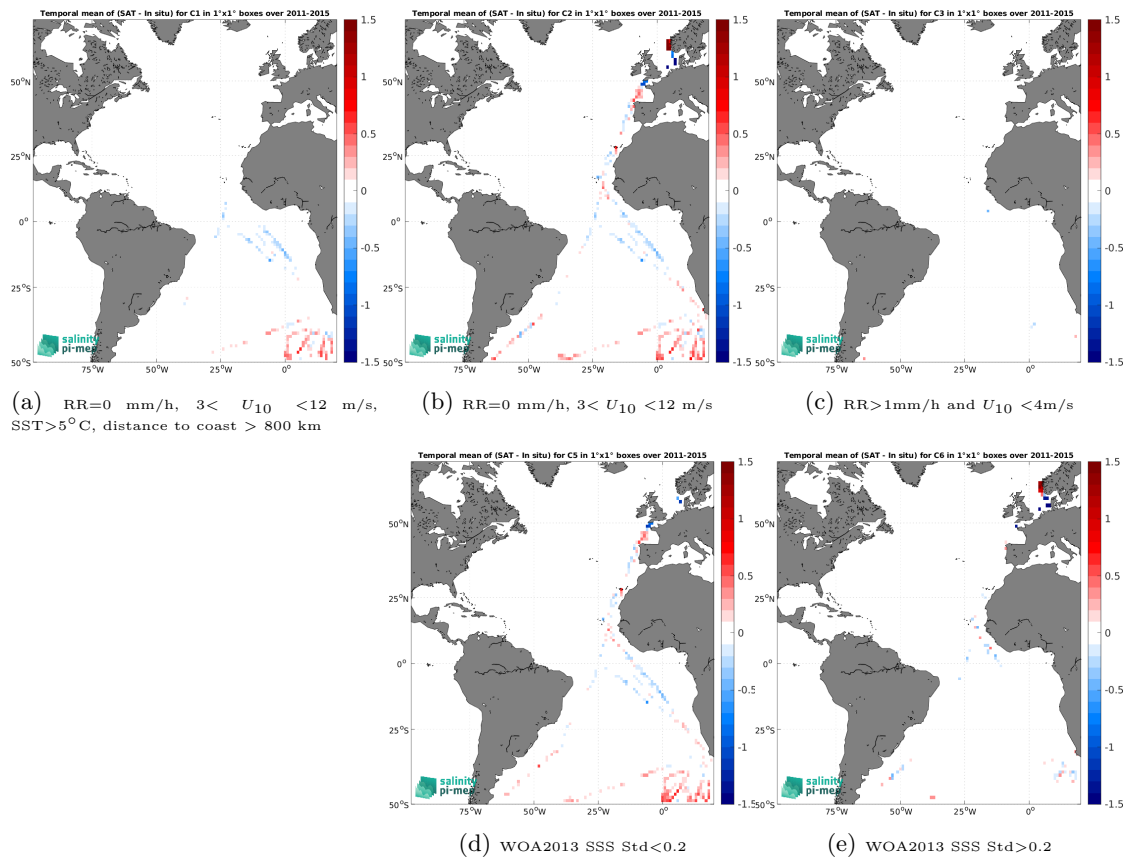
Figure 14: Temporal mean gridded over spatial boxes of size 1^\circ \times 1^\circ of \Delta\text{SSS} (Aquarius SSS L3 CAP v5 - Monthly (JPL) - TSG (Polarstern)) for 5 different subdatasets corresponding to:RR=0 mm/h, 3 < U_{10} < 12 m/s, SST>5°C, distance to coast > 800 km (a), RR=0 mm/h, 3 < U_{10} < 12 m/s (b), RR>1mm/h and U_{10} < 4 m/s (c), WOA2013 SSS Std<0.2 (d), WOA2013 SSS Std>0.2 (e).
