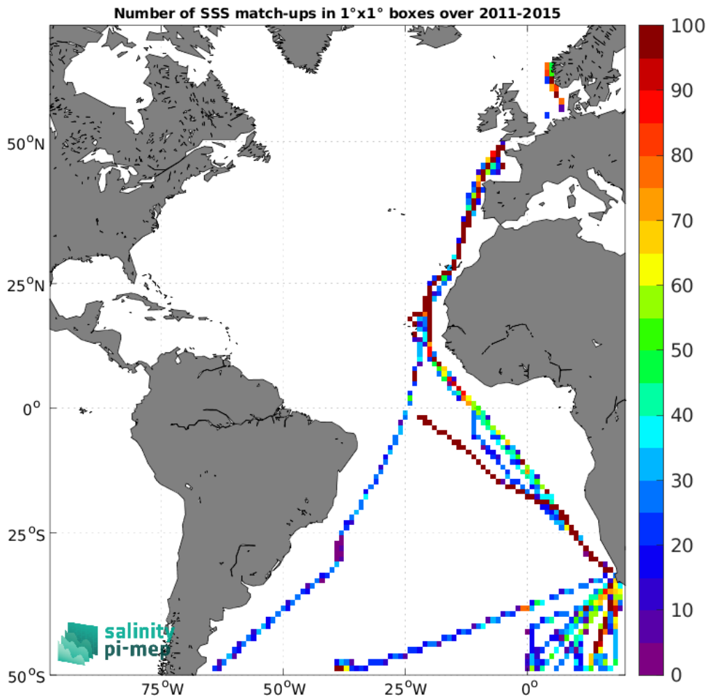
Figure 5: Number of SSS match-ups between TSG (Polarstern) SSS and the Aquarius SSS L3 CAP v5 - Monthly (JPL) SSS product for the Atlantic Ocean Pi-MEP region over 1^\circ \times 1^\circ boxes and for the full satellite product period.
