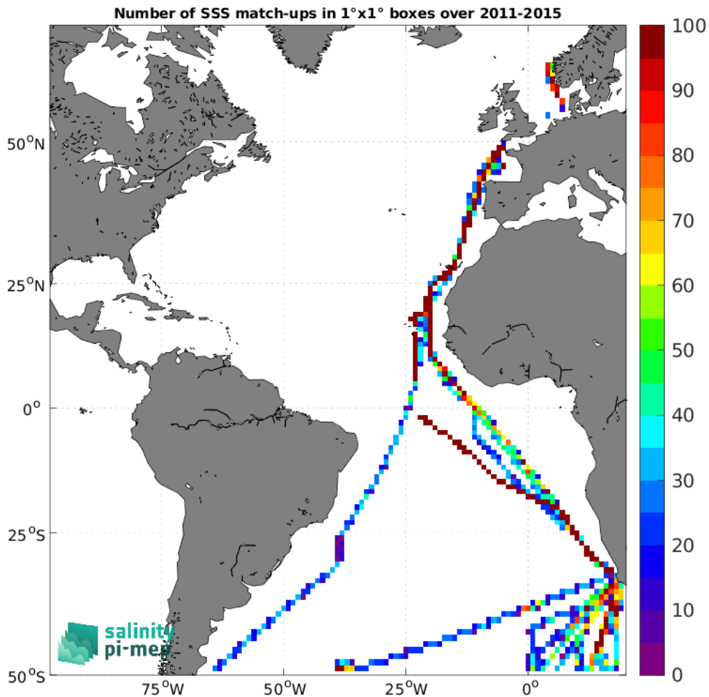
Figure 4: Number of SSS match-ups between TSG (Polarstern) SSS and the Aquarius SSS L3 CAP v5 - Monthly (JPL) SSS product for the Atlantic Ocean Pi-MEP region over 1^\circ \times 1^\circ boxes and for the full satellite product period.
