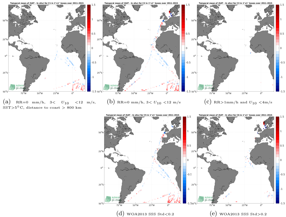
Figure 12: Temporal mean gridded over spatial boxes of size 1^\circ \times 1^\circ of \Delta SSS (Aquarius SSS L3 CAP v5 - Monthly (JPL) - TSG (Polarstern)) for 5 different subdatasets corresponding to:RR=0 mm/h, 3 < U_{10} < 12 m/s, SST >5^\circ\text{C} , distance to coast > 800 km (a), RR=0 mm/h, 3 < U_{10} < 12 m/s (b), RR >1 mm/h and U_{10} < 4 m/s (c), WOA2013 SSS Std <0.2 (d), WOA2013 SSS Std >0.2 (e).
