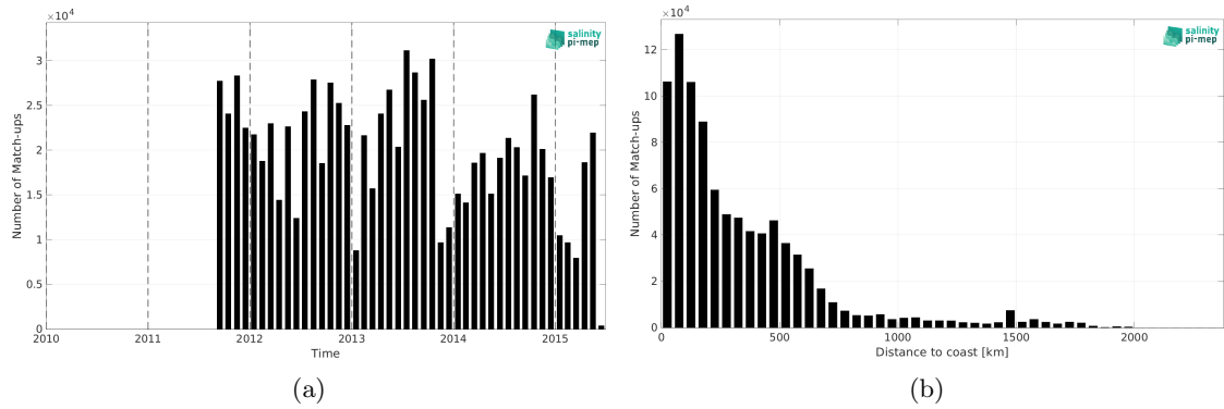
Figure 2: Number of match-ups between TSG (LEGOS-DM) and Aquarius SSS L3 CAP v5 - Monthly (JPL) SSS as a function of time (a) and as function of the distance to coast (b) over the Atlantic Ocean Pi-MEP region and for the full satellite product period.
