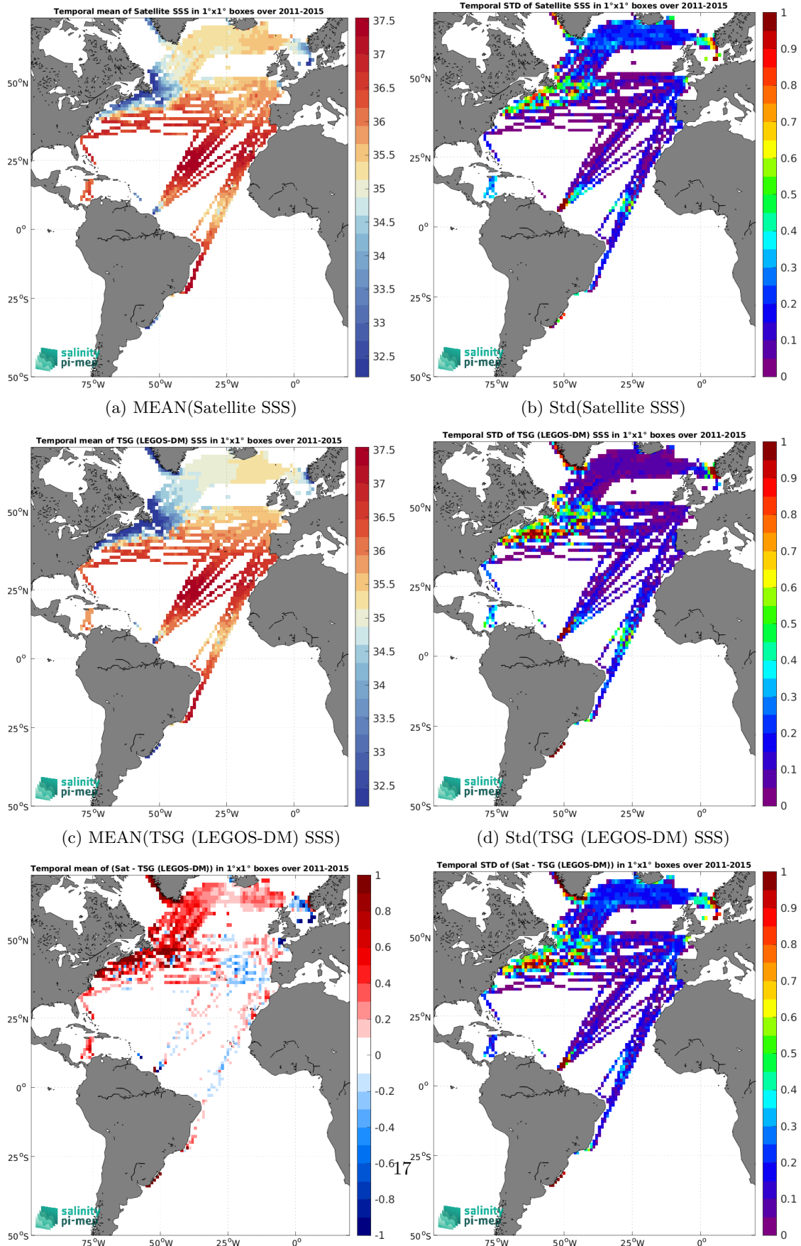
Figure 7: Temporal mean (left) and Std (right) of SSS from Aquarius SSS L3 CAP v5 - Monthly (JPL) (top), TSG (LEGOS-DM) (middle), and of \Delta SSS (Satellite - TSG (LEGOS-DM)). Only match-up pairs are used to generate these maps.
