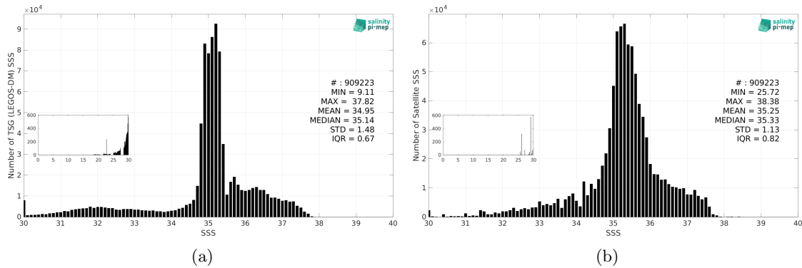
Figure 3: Histograms of SSS from TSG (LEGOS-DM) (a) and Aquarius SSS L3 CAP v5 - Monthly (JPL) (b) considering all match-up pairs per bins of 0.1 over the Atlantic Ocean Pi-MEP region and for the full satellite product period.
