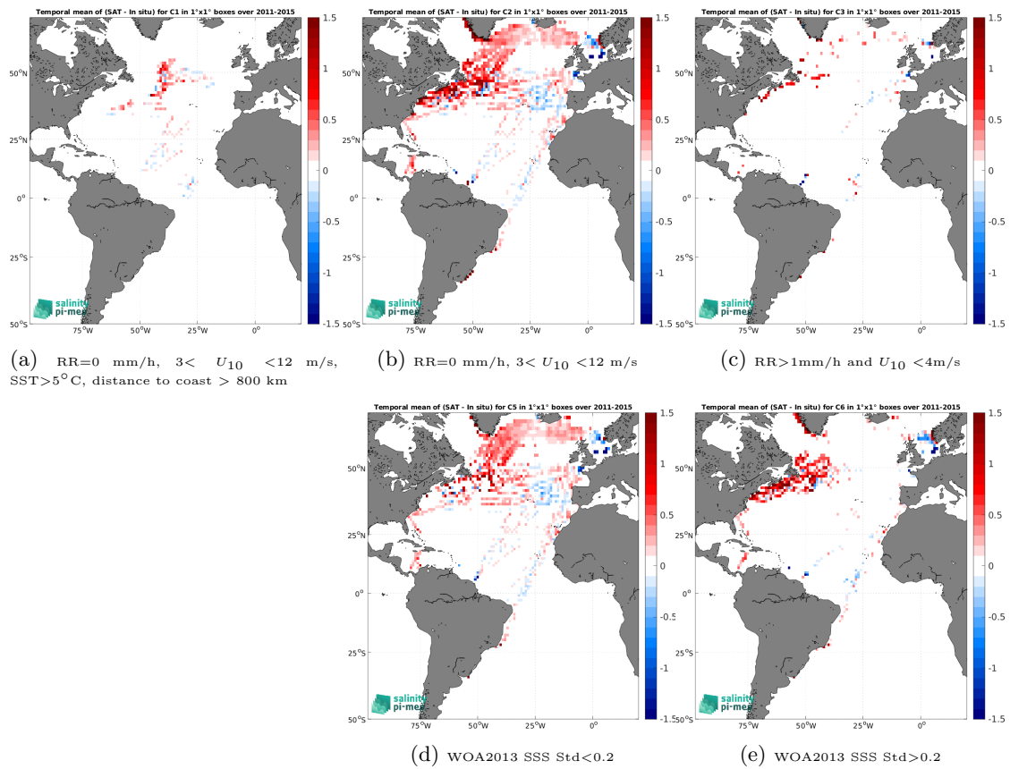
Figure 14: Temporal mean gridded over spatial boxes of size 1^\circ \times 1^\circ of \Delta\text{SSS} (Aquarius SSS L3 CAP v5 - Monthly (JPL) - TSG (LEGOS-DM)) for 5 different subdatasets corresponding to:RR=0 mm/h, 3 < U_{10} < 12 m/s, SST >5^\circ\text{C} , distance to coast > 800 km (a), RR=0 mm/h, 3 < U_{10} < 12 m/s (b), RR >1 mm/h and U_{10} < 4 m/s (c), WOA2013 SSS Std <0.2 (d), WOA2013 SSS Std >0.2 (e).
