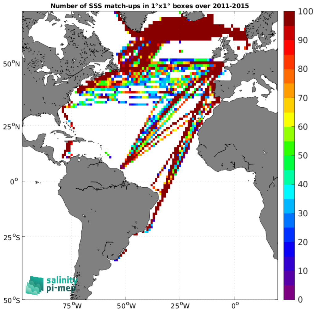
Figure 5: Number of SSS match-ups between TSG (LEGOS-DM) SSS and the Aquarius SSS L3 CAP v5 - Monthly (JPL) SSS product for the Atlantic Ocean Pi-MEP region over 1^\circ \times 1^\circ boxes and for the full satellite product period.
