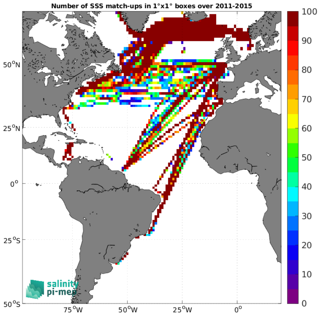
Figure 4: Number of SSS match-ups between TSG (LEGOS-DM) SSS and the Aquarius SSS L3 CAP v5 - Monthly (JPL) SSS product for the Atlantic Ocean Pi-MEP region over 1°×1° boxes and for the full satellite product period.
