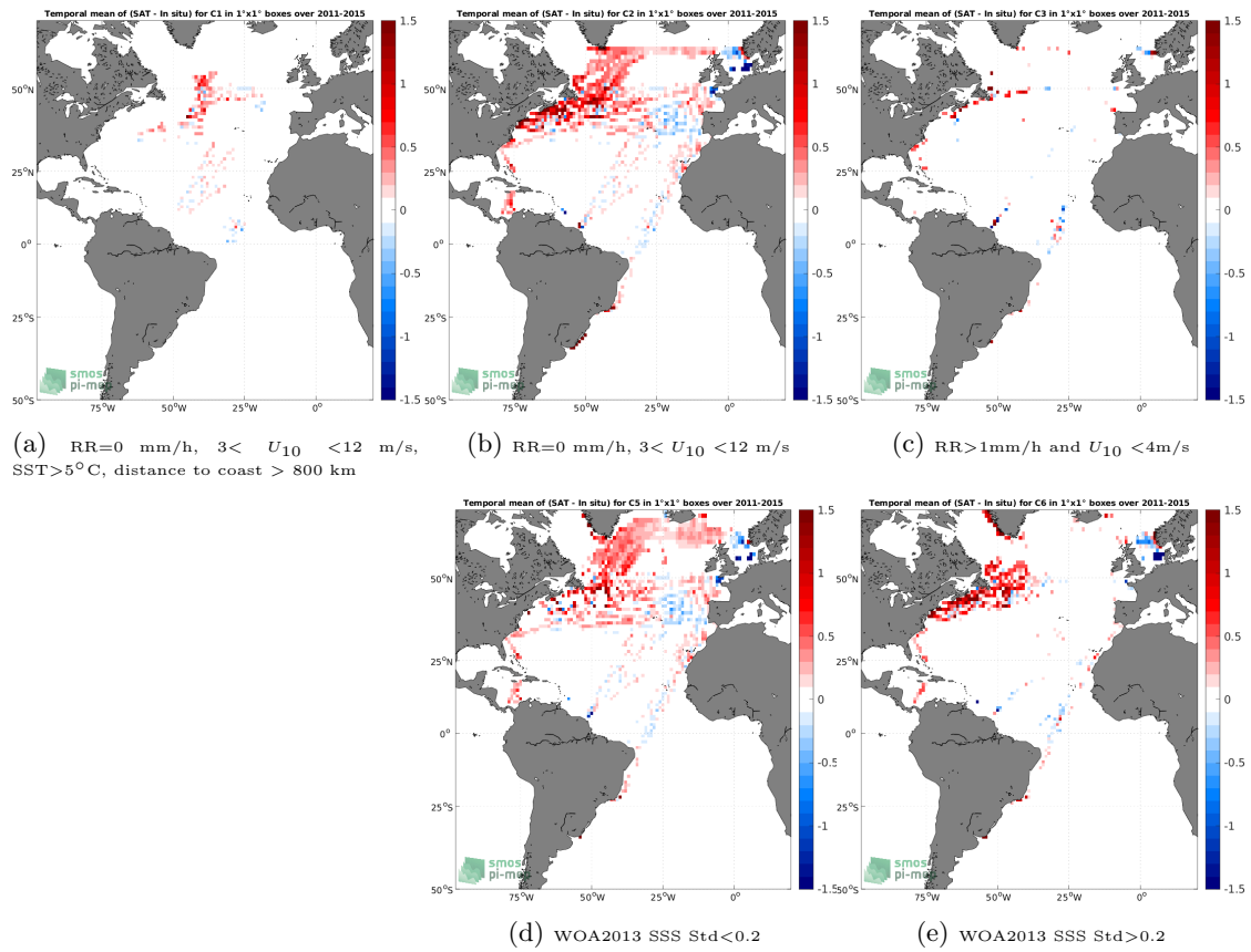
Figure 12: Temporal mean gridded over spatial boxes of size 1^\circ \times 1^\circ of \Delta SSS (Aquarius SSS L3 CAP v5 - Monthly (JPL) - TSG (LEGOS-DM)) for 5 different subdatasets corresponding to:RR=0 mm/h, 3 < U_{10} < 12 m/s, SST >5^\circ\text{C} , distance to coast > 800 km (a), RR=0 mm/h, 3 < U_{10} < 12 m/s (b), RR >1 mm/h and U_{10} < 4 m/s (c), WOA2013 SSS Std <0.2 (d), WOA2013 SSS Std >0.2 (e).
