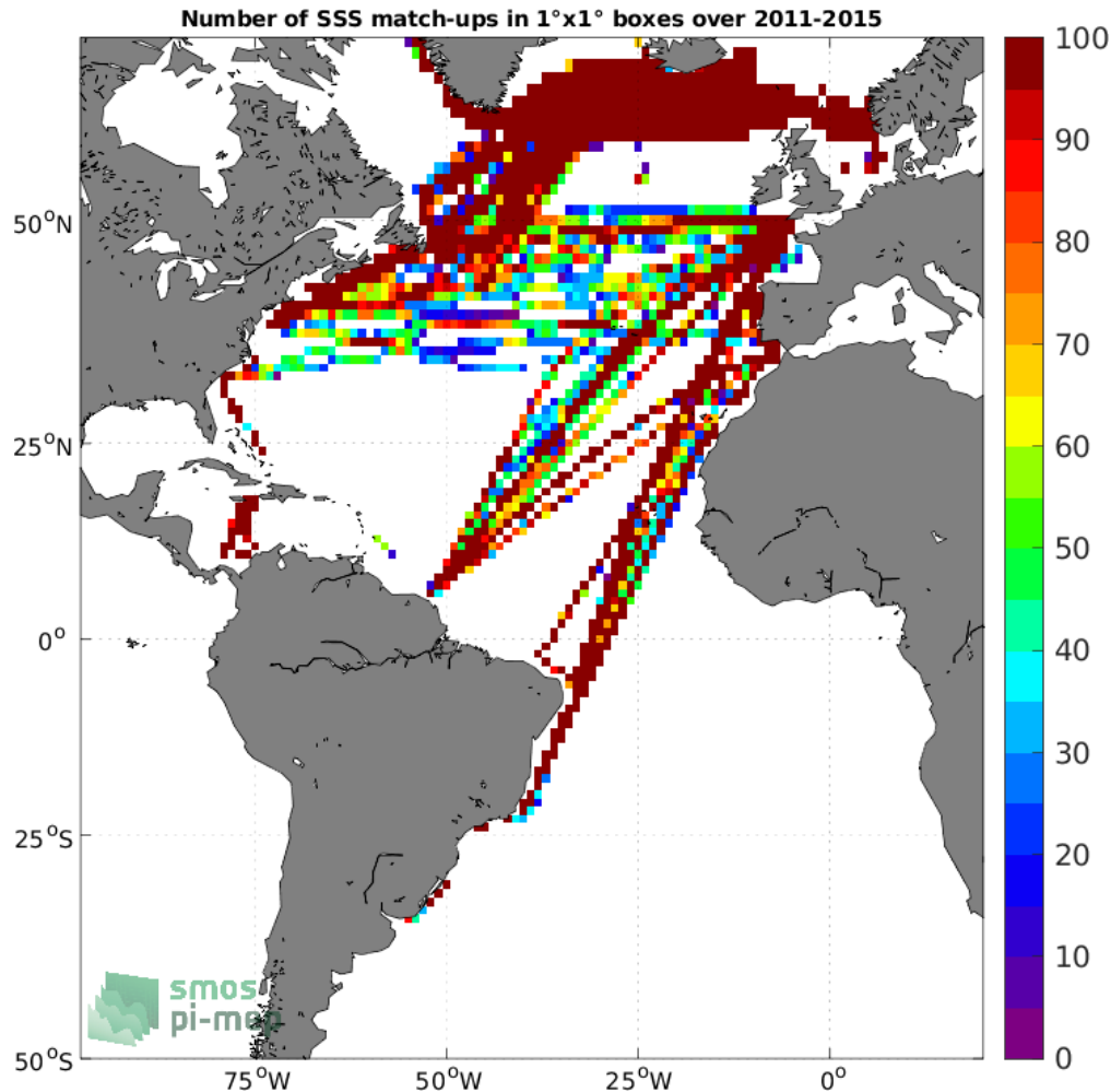
Figure 4: Number of SSS match-ups between TSG (LEGOS-DM) SSS and the Aquarius SSS L3 CAP v5 - Monthly (JPL) SSS product for the Atlantic Ocean Pi-MEP region over 1^\circ \times 1^\circ boxes and for the full satellite product period.
