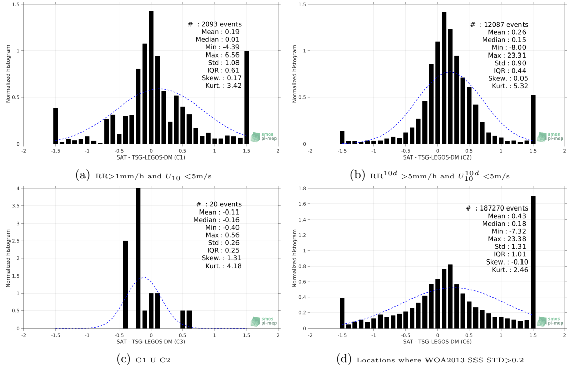
Figure 13: Normalized histogram of \Delta SSS (Aquarius-L3-JPL-V5-MONTHLY - TSG-LEGOS-DM) for 6 different subdatasets corresponding to: RR > 1\text{mm/h} and U_{10} < 5\text{m/s} (a), RR^{10d} > 5\text{mm/h} and U_{10}^{10d} < 5\text{m/s} (b), C1 U C2 (c), Locations where WOA2013 SSS STD > 0.2 (d).
