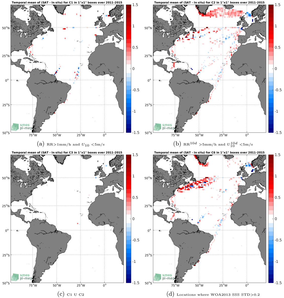
Figure 12: Temporal mean gridded over spatial boxes of size 1^\circ \times 1^\circ of \Delta SSS (Aquarius-L3-JPL-V5-MONTHLY - TSG-LEGOS-DM) for 4 different subdatasets corresponding to:RR>1mm/h and U_{10} < 5\text{m/s} (a), RR^{10d} > 5\text{mm/h} and U_{10}^{10d} < 5\text{m/s} (b), C1 U C2 (c),Locations where WOA2013 SSS STD>0.2 (d).
