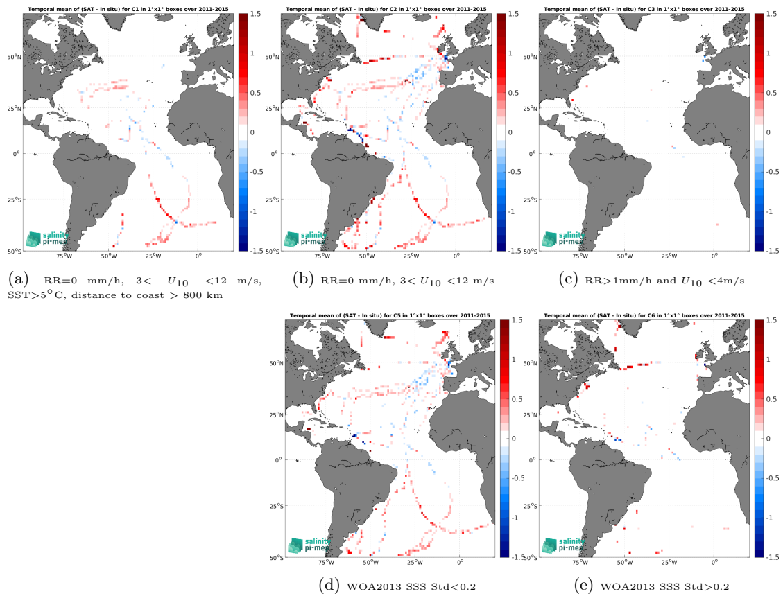
Figure 14: Temporal mean gridded over spatial boxes of size 1^\circ \times 1^\circ of \Delta SSS (Aquarius SSS L3 CAP v5 - Monthly (JPL) - TSG (GOSUD-Sailing-ship)) for 5 different subdatasets corresponding to:RR=0 mm/h, 3 < U_{10} < 12 m/s, SST >5^\circ\text{C} , distance to coast > 800 km (a), RR=0 mm/h, 3 < U_{10} < 12 m/s (b), RR >1 mm/h and U_{10} < 4 m/s (c), WOA2013 SSS Std <0.2 (d), WOA2013 SSS Std >0.2 (e).
