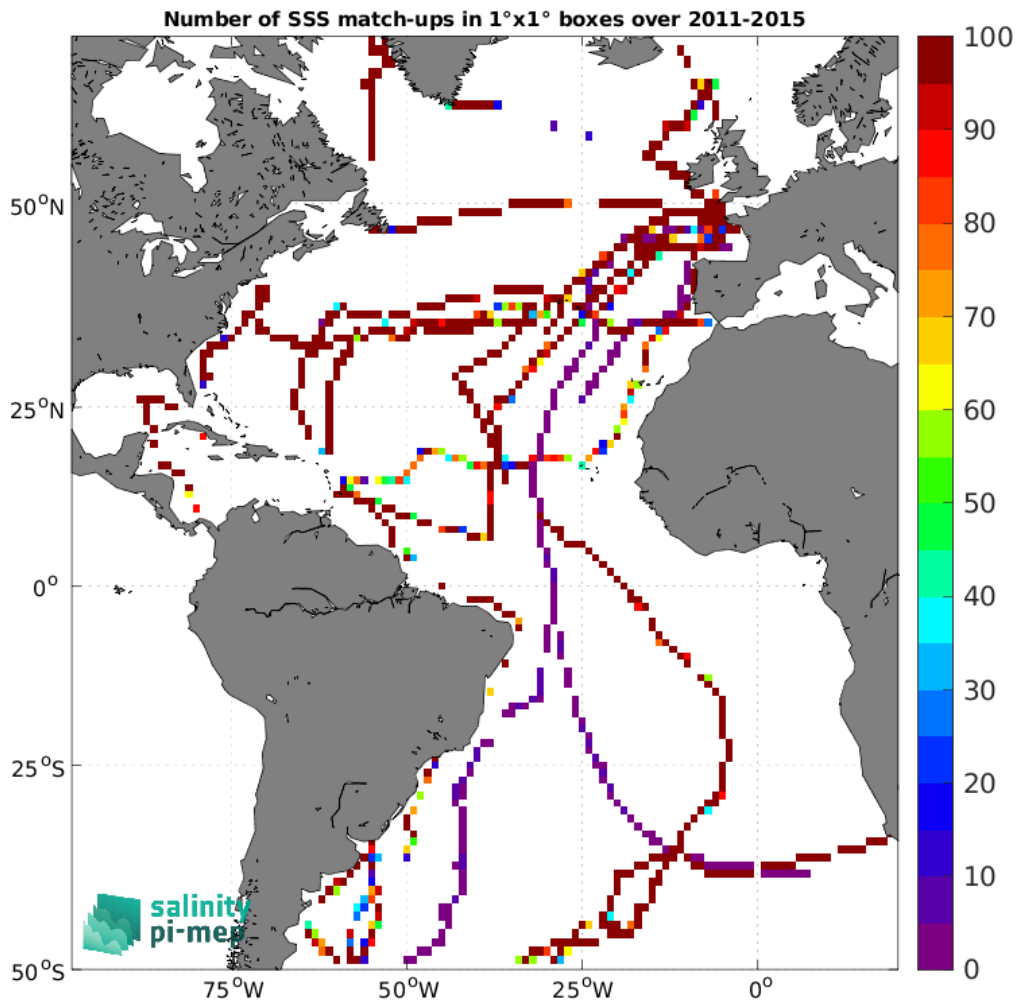
Figure 5: Number of SSS match-ups between TSG (GOSUD-Sailing-ship) SSS and the Aquarius SSS L3 CAP v5 - Monthly (JPL) SSS product for the Atlantic Ocean Pi-MEP region over 1^\circ \times 1^\circ boxes and for the full satellite product period.
