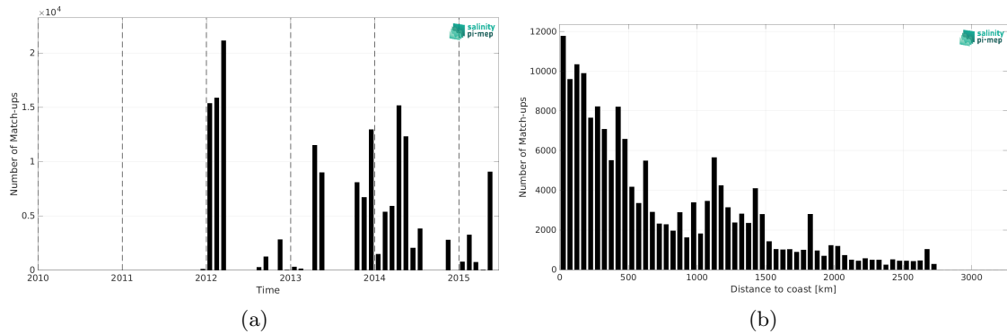
Figure 2: Number of match-ups between TSG (GOSUD-Sailing-ship) and Aquarius SSS L3 CAP v5 - Monthly (JPL) SSS as a function of time (a) and as function of the distance to coast (b) over the Atlantic Ocean Pi-MEP region and for the full satellite product period.
