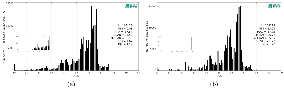
Figure 3: Histograms of SSS from TSG (GOSUD-Sailing-ship) (a) and Aquarius SSS L3 CAP v5 - Monthly (JPL) (b) considering all match-up pairs per bins of 0.1 over the Atlantic Ocean Pi-MEP region and for the full satellite product period.
