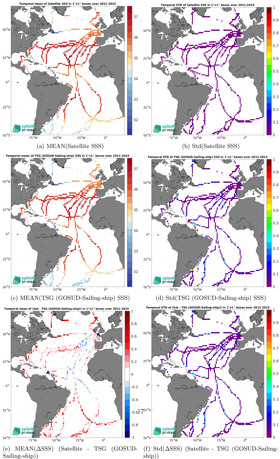
Figure 7: Temporal mean (left) and Std (right) of SSS from Aquarius SSS L3 CAP v5 - Monthly (JPL) (top), TSG (GOSUD-Sailing-ship) (middle), and of \Delta\text{SSS} (Satellite - TSG (GOSUD-Sailing-ship)). Only match-up pairs are used to generate these maps.
