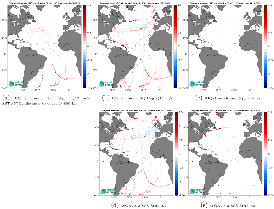
Figure 14: Temporal mean gridded over spatial boxes of size 1^\circ \times 1^\circ of \Delta\text{SSS} (Aquarius SSS L3 CAP v5 - Monthly (JPL) - TSG (GOSUD-Sailing-ship)) for 5 different subdatasets corresponding to:RR=0 mm/h, 3 < U_{10} < 12 m/s, SST >5^\circ\text{C} , distance to coast > 800 km (a), RR=0 mm/h, 3 < U_{10} < 12 m/s (b), RR >1 mm/h and U_{10} < 4 m/s (c), WOA2013 SSS Std <0.2 (d), WOA2013 SSS Std >0.2 (e).
