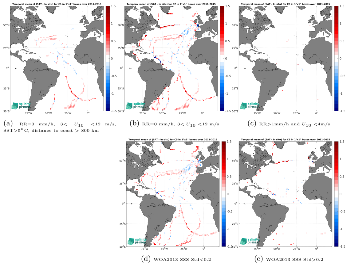
Figure 12: Temporal mean gridded over spatial boxes of size 1^\circ \times 1^\circ of \Delta\text{SSS} (Aquarius SSS L3 CAP v5 - Monthly (JPL) - TSG (GOSUD-Sailing-ship)) for 5 different subdatasets corresponding to:RR=0 mm/h, 3 < U_{10} < 12 m/s, SST >5^\circ\text{C} , distance to coast > 800 km (a), RR=0 mm/h, 3 < U_{10} < 12 m/s (b), RR >1 mm/h and U_{10} < 4 m/s (c), WOA2013 SSS Std <0.2 (d), WOA2013 SSS Std >0.2 (e).
