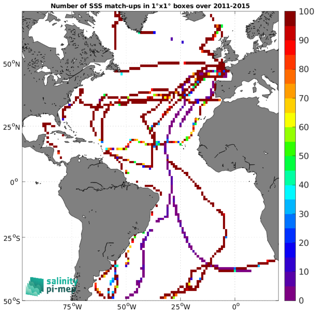
Figure 4: Number of SSS match-ups between TSG (GOSUD-Sailing-ship) SSS and the Aquarius SSS L3 CAP v5 - Monthly (JPL) SSS product for the Atlantic Ocean Pi-MEP region over 1^\circ \times 1^\circ boxes and for the full satellite product period.
