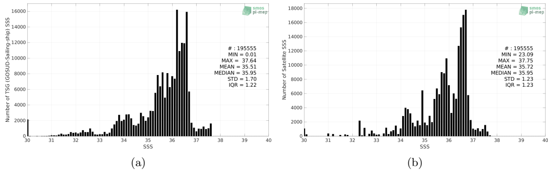
Figure 2: Histograms of SSS from TSG (GOSUD-Sailing-ship) (a) and Aquarius SSS L3 CAP v5 - Monthly (JPL) (b) considering all match-up pairs per bins of 0.1 over the Atlantic Ocean Pi-MEP region and for the full satellite product period.
