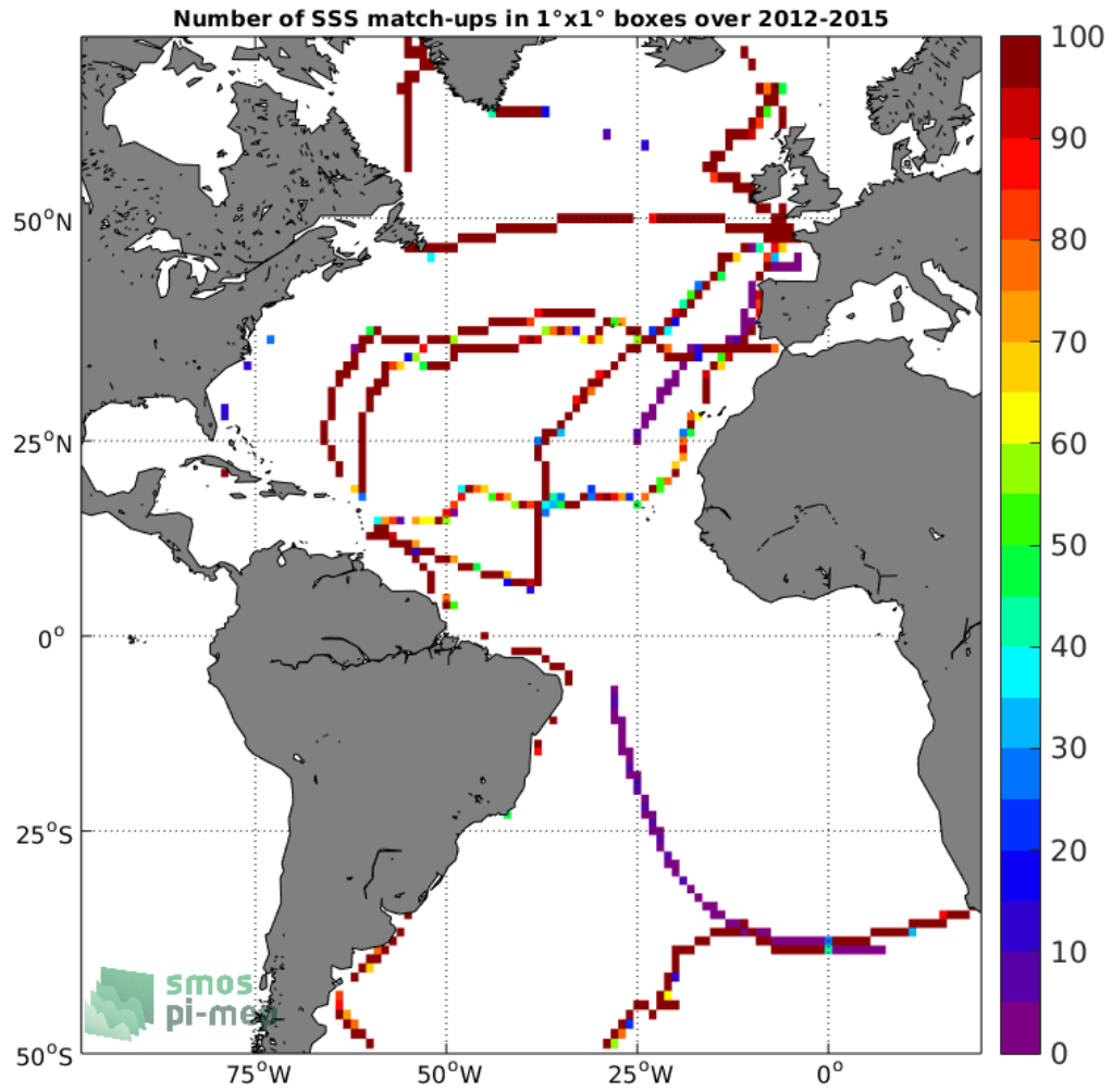
Figure 4: Number of SSS match-ups between TSG-GOSUD-Sailing-ship SSS and the Aquarius-L3-JPL-V5-MONTHLY SSS product for the Atlantic Ocean Pi-MEP region over 1^\circ \times 1^\circ boxes and for the full satellite product period.
