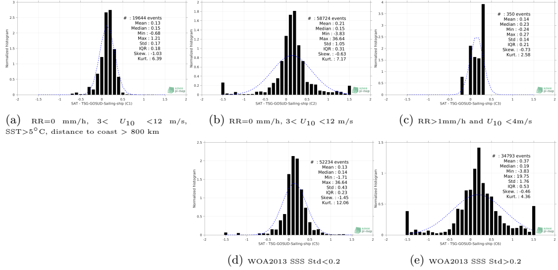
Figure 13: Normalized histogram of \Delta\text{SSS} (Aquarius-L3-JPL-V5-MONTHLY - TSG-GOSUD-Sailing-ship) for 5 different subdatasets corresponding to: RR=0 mm/h, 3 < U_{10} < 12 m/s, SST > 5^{\circ}\text{C} , distance to coast > 800 km (a), RR=0 mm/h, 3 < U_{10} < 12 m/s (b), RR > 1\text{mm/h} and U_{10} < 4\text{m/s} (c), WOA2013 SSS Std < 0.2 (d), WOA2013 SSS Std > 0.2 (e).
