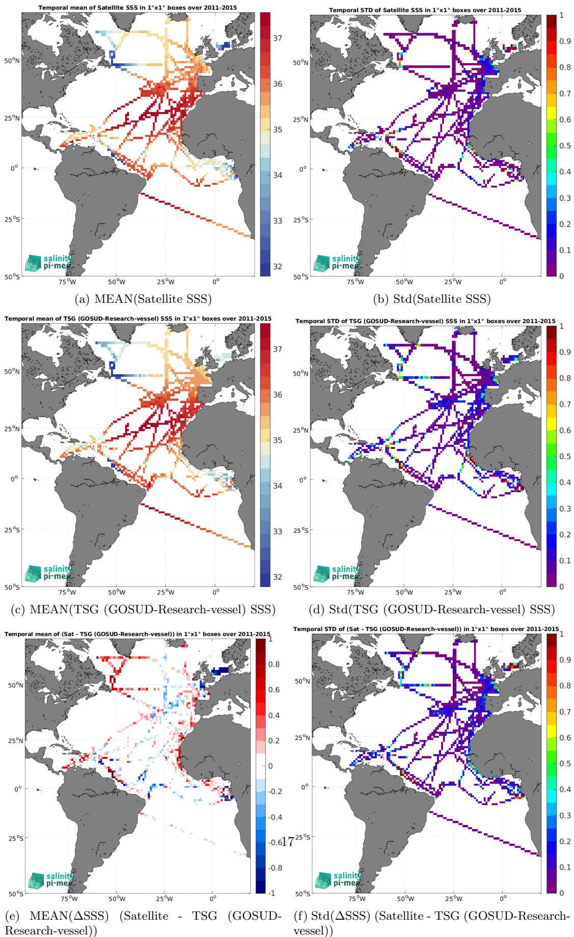
Figure 7: Temporal mean (left) and Std (right) of SSS from Aquarius SSS L3 CAP v5 - Monthly (JPL) (top), TSG (GOSUD-Research-vessel) (middle), and of \Delta SSS (Satellite - TSG (GOSUD-Research-vessel)). Only match-up pairs are used to generate these maps.
