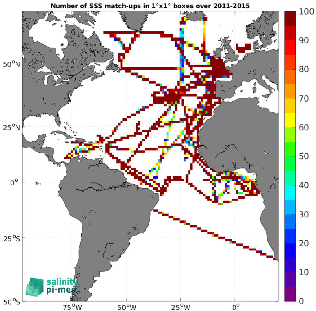
Figure 4: Number of SSS match-ups between TSG (GOSUD-Research-vessel) SSS and the Aquarius SSS L3 CAP v5 - Monthly (JPL) SSS product for the Atlantic Ocean Pi-MEP region over 1^{\circ} \times 1^{\circ} boxes and for the full satellite product period.
