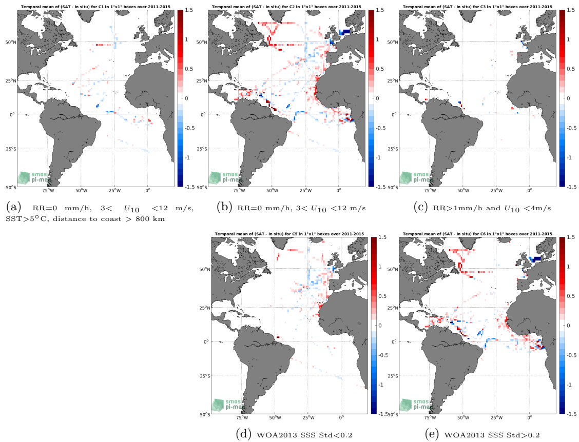
Figure 12: Temporal mean gridded over spatial boxes of size 1^\circ \times 1^\circ of \Delta SSS (Aquarius SSS L3 CAP v5 - Monthly (JPL) - TSG (GOSUD-Research-vessel)) for 5 different subdatasets corresponding to:RR=0 mm/h, 3 < U_{10} < 12 m/s, SST>5°C, distance to coast > 800 km (a), RR=0 mm/h, 3 < U_{10} < 12 m/s (b), RR>1mm/h and U_{10} < 4 m/s (c), WOA2013 SSS Std<0.2 (d), WOA2013 SSS Std>0.2 (e).
