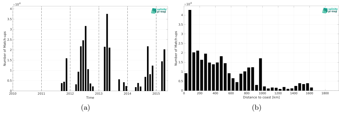
Figure 2: Number of match-ups between TSG (CSIC-UTM) and Aquarius SSS L3 CAP v5 - Monthly (JPL) SSS as a function of time (a) and as function of the distance to coast (b) over the Atlantic Ocean Pi-MEP region and for the full satellite product period.
