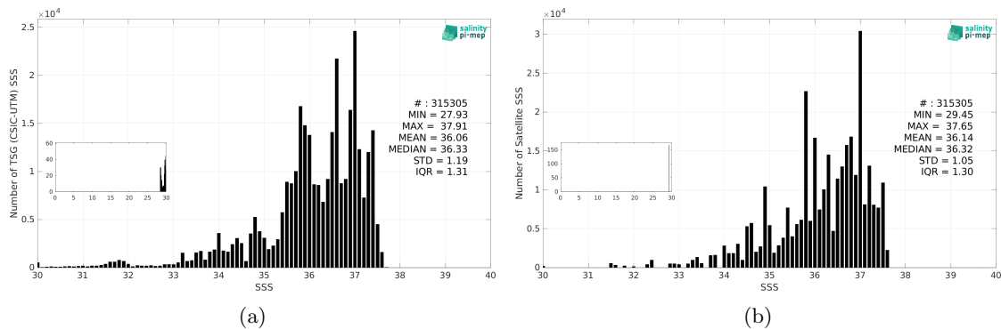
Figure 3: Histograms of SSS from TSG (CSIC-UTM) (a) and Aquarius SSS L3 CAP v5 - Monthly (JPL) (b) considering all match-up pairs per bins of 0.1 over the Atlantic Ocean Pi-MEP region and for the full satellite product period.
